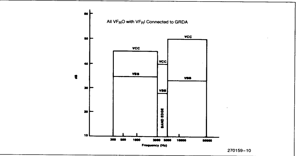
Figure 10. Receive Filter
