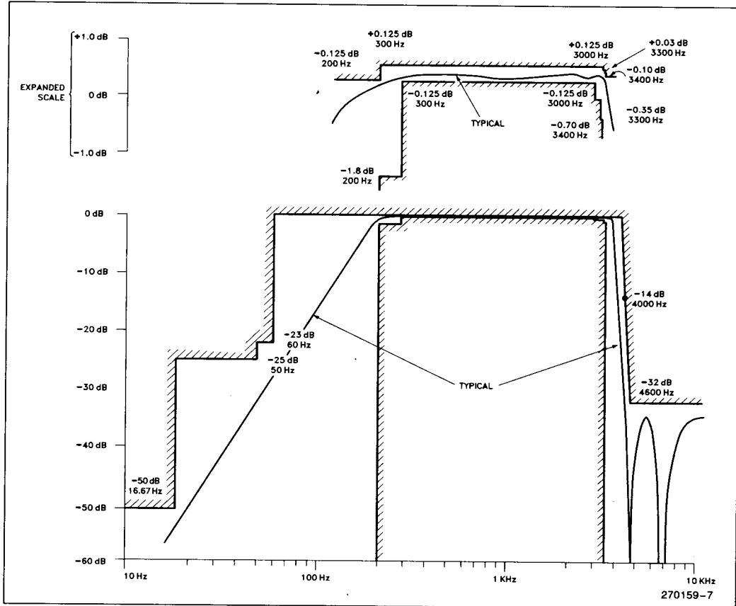
Figure 7. Transmit Filter
