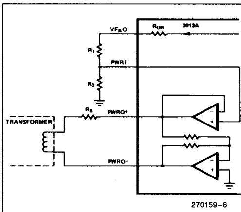
Figure 6. Typical Connection of Output Driver Amplifier
