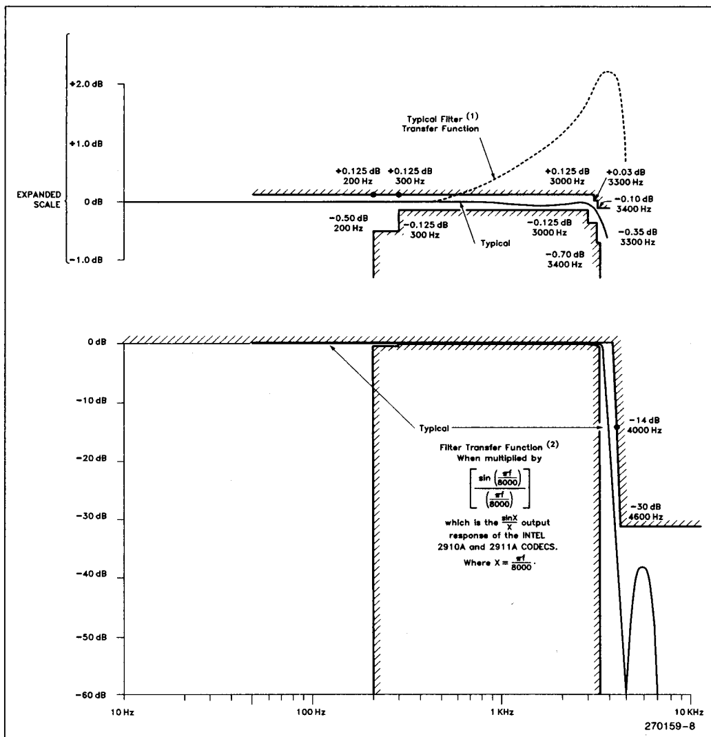
Figure 8. Receive Filter
