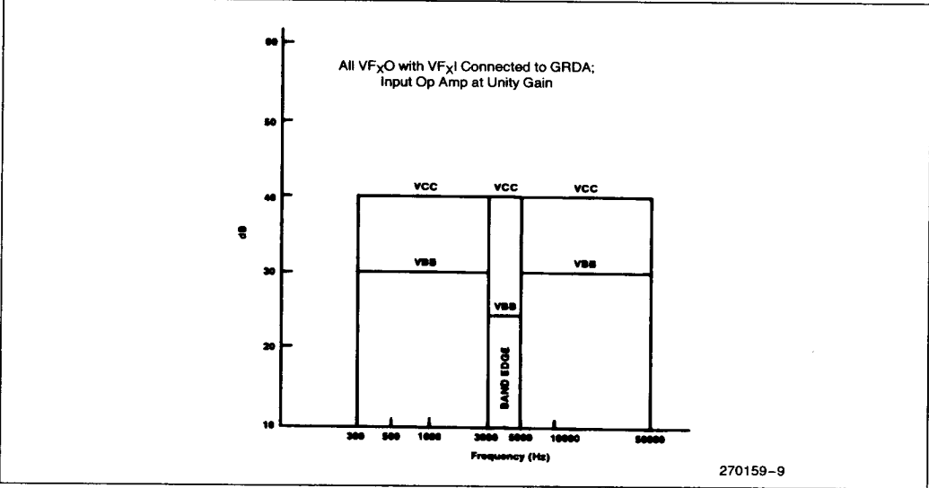
Figure 9. Transmit Filter
