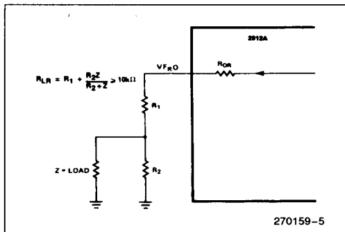
Figure 5. Receive Filter Output Gain Adjustment
