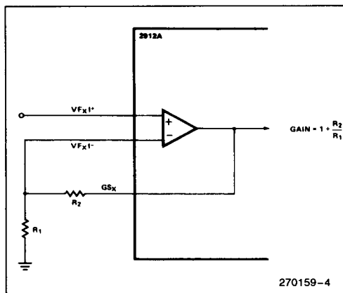
Figure 4. Transmit Filter Gain Adjustment
