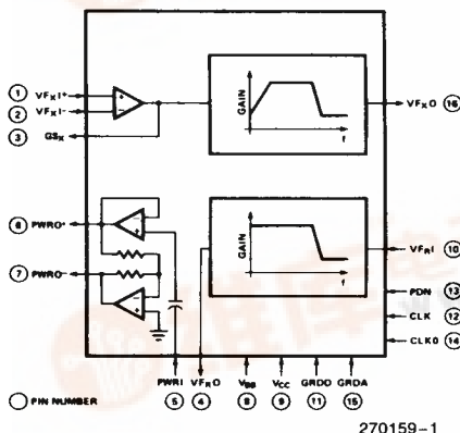
Figure 1. Block Diagram
