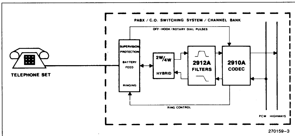
Figure 3. Typical Line Termination
