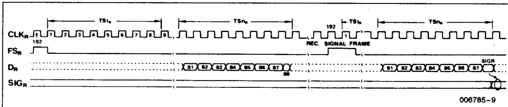
Figure 9. Receive 8th Bit Signaling
