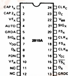
Figure 2. Pin Configuration
