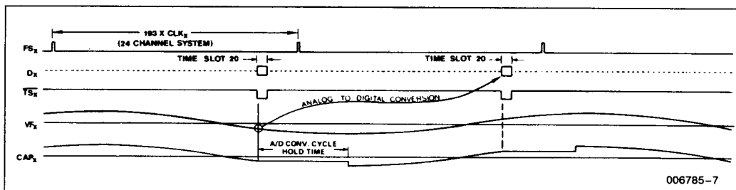
Figure 7. Transmit Encoding
