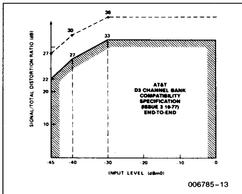
Figure 13. Signal/Total Distortion Ratio (Half-Channel)
