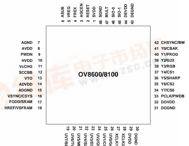
Figure 1. OV8610/OV8110 Pin Diagram
