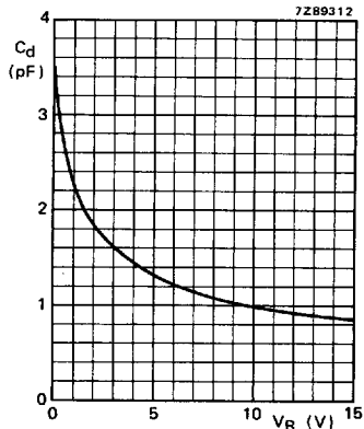
Fig. 2 Diode capacitance as a function of continuous reverse voltage; f = 1 MHz; T_j = 25 °C; typical values.
