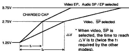
Fig.21 Charging capacitor voltage characteristic
