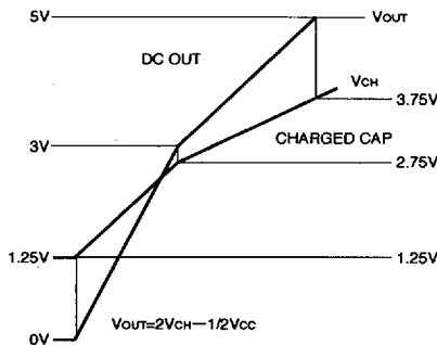
Fig. 22 Charging capacitor vs. DC output characteristic
