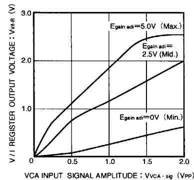
Fig. 18 V/I register output voltage vs VCA input signal amplitude
