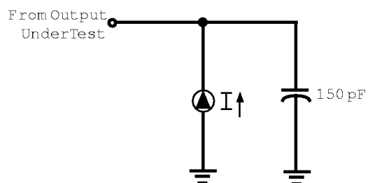
Figure 7. Test Load Diagram
