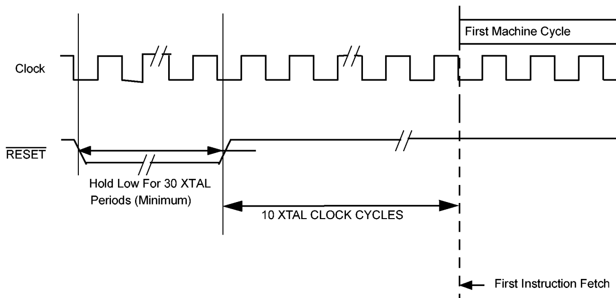
Figure 9. Reset Timing
