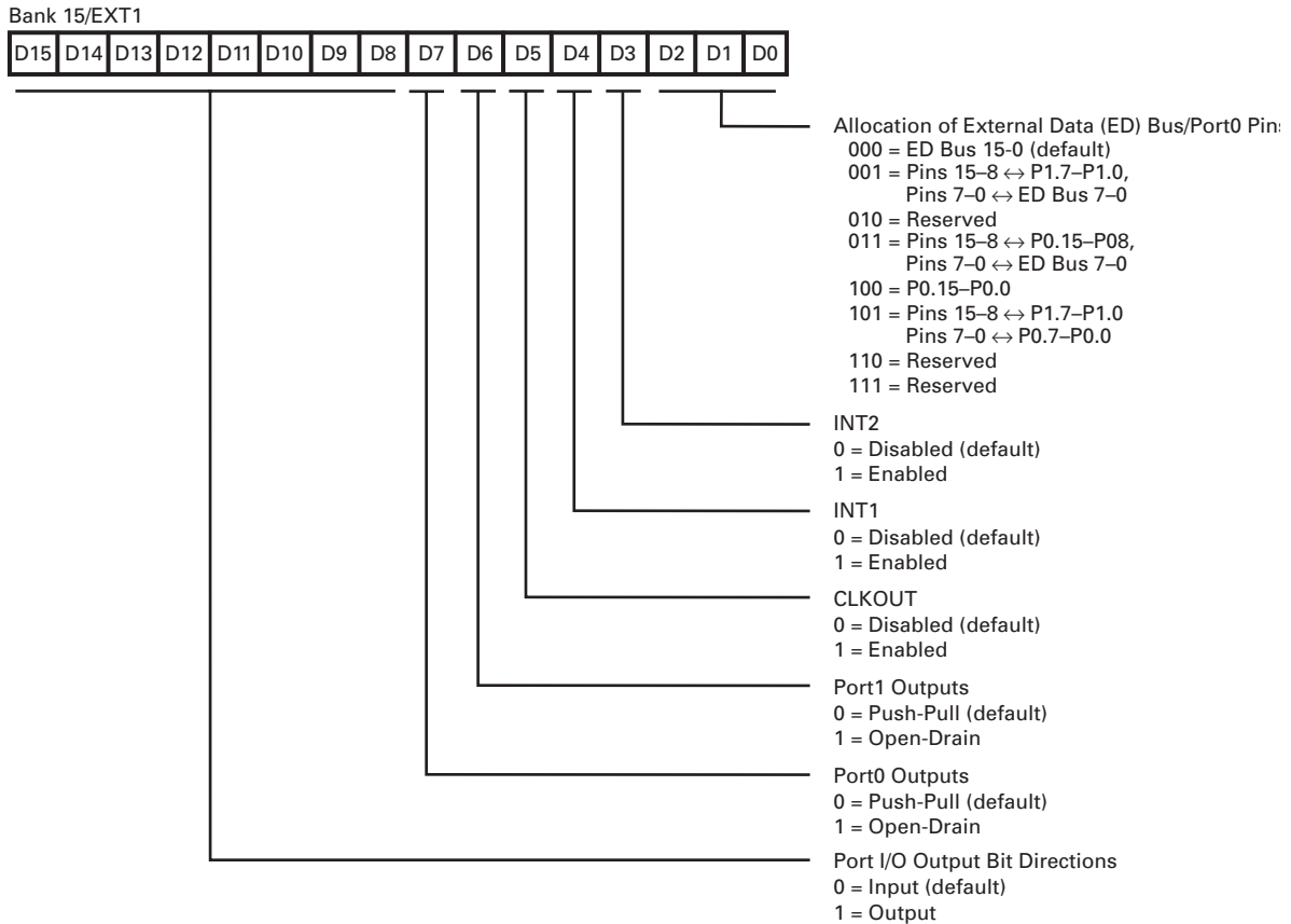
Figure 26. Bank15/EXT1 Register
