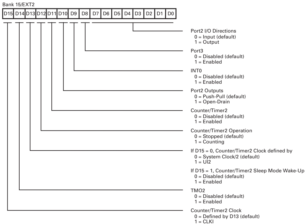
Figure 27. Bank15/EXT2 Register
