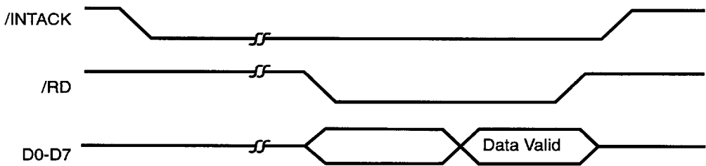
Figure 14. Interrupt Acknowledge Cycle Timing
