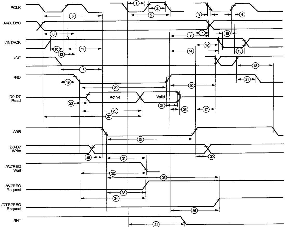
Figure 20. Read and Write Timing
