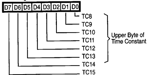
Write Register 13
