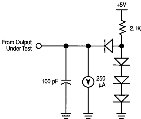
Figure 18. Standard Test Load
