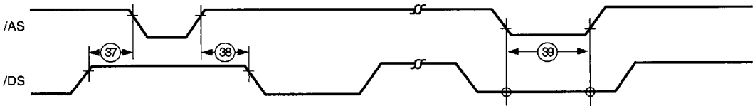
Figure 28. Rest Timing
