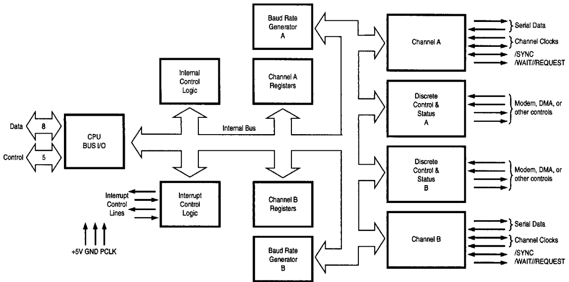
Figure 8. Block Diagram of SCC Architecture
