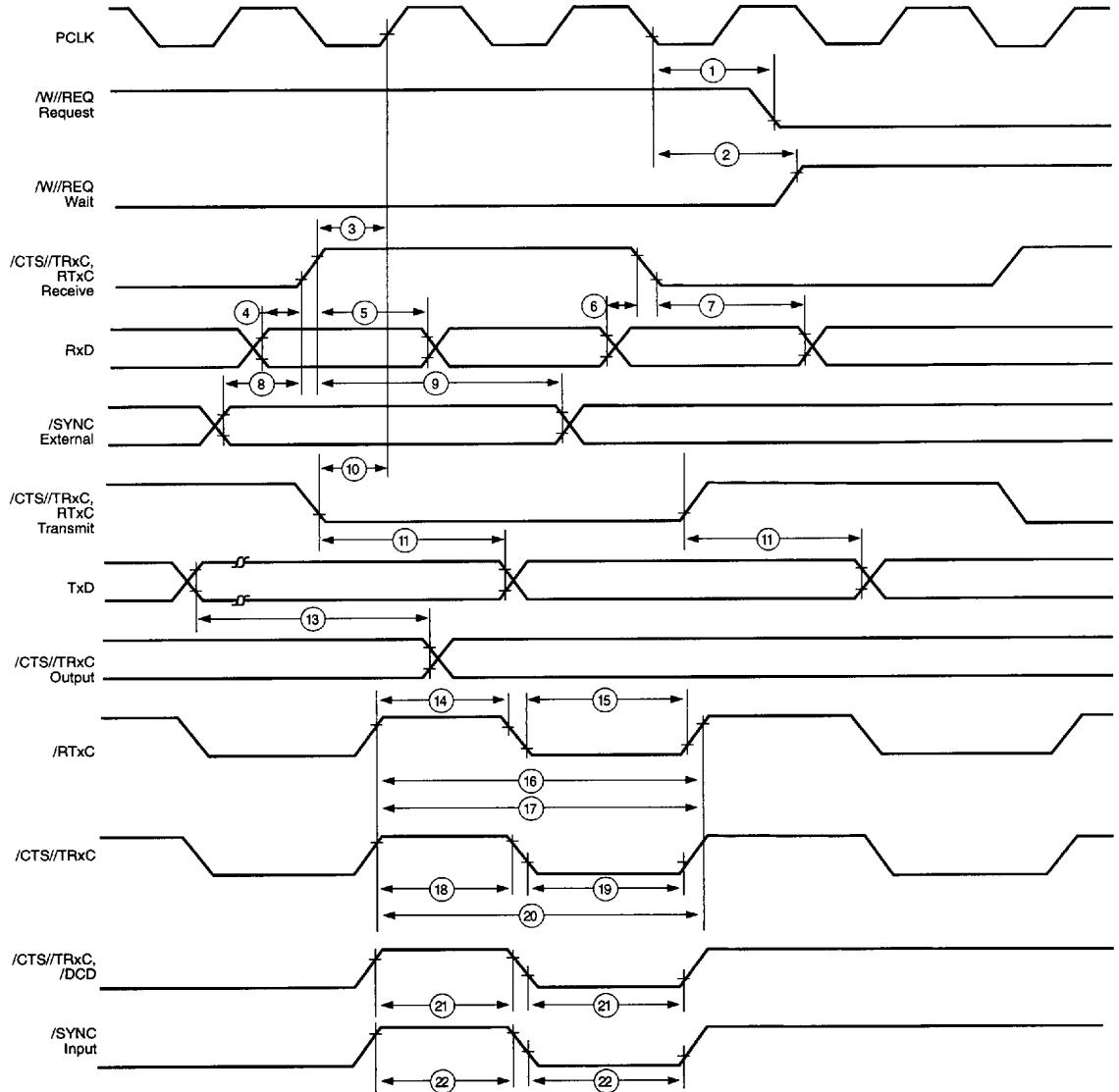
Figure 24. 28530 General Timing Diagram
