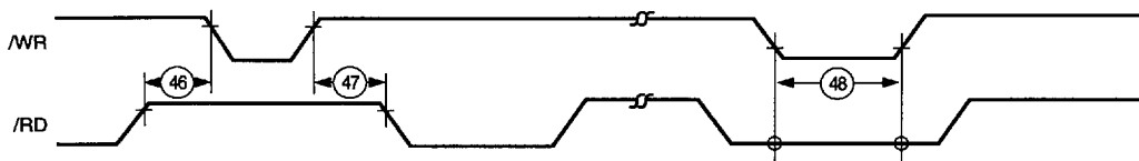
Figure 22. Reset Timing
