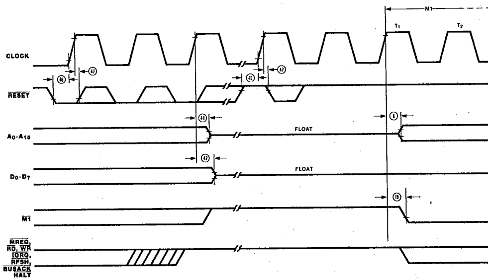
Figure 12. Reset Cycle
