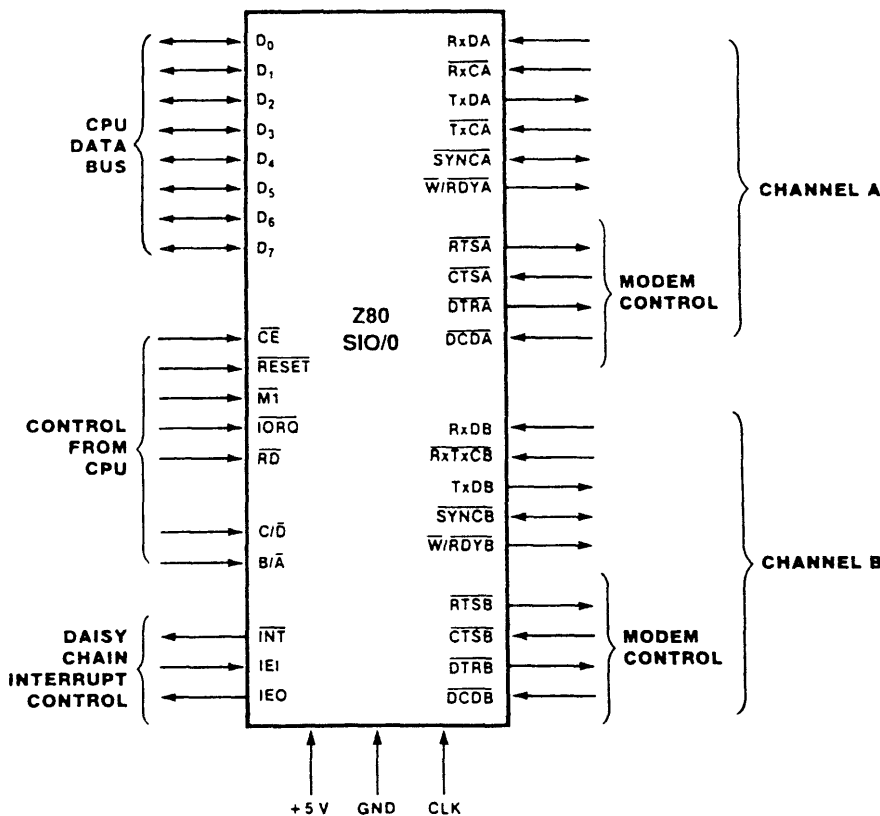
Figure 5. Pin Functions
