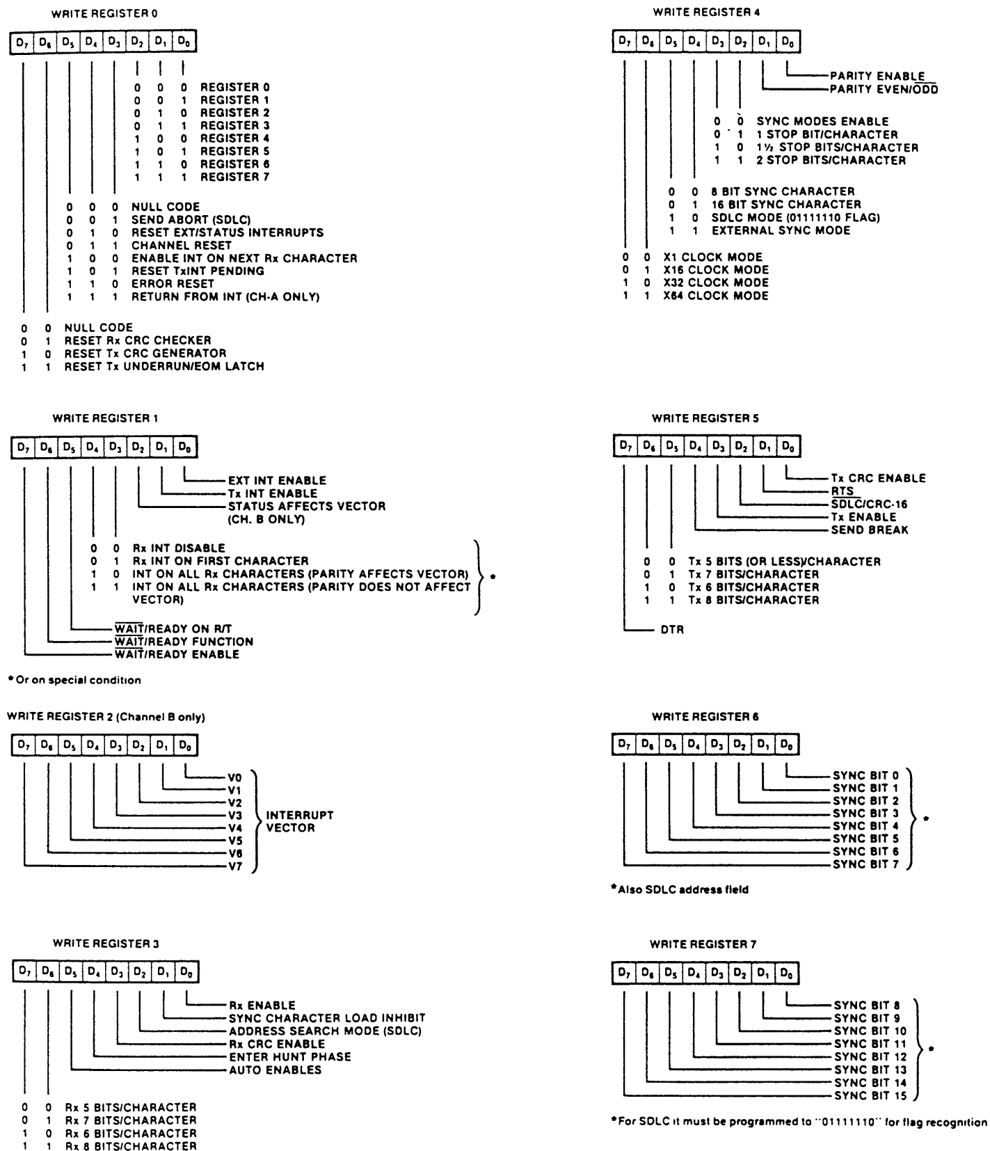
Figure 14. Write Register Bit Functions
