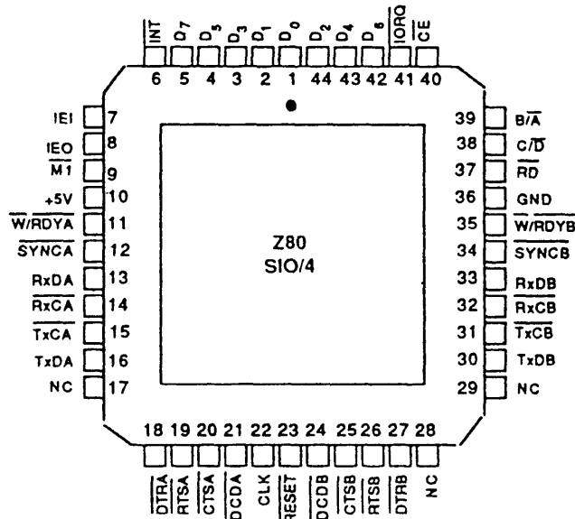
Figure 7a. 44-pin Chip Carrier, Pin Assignments
