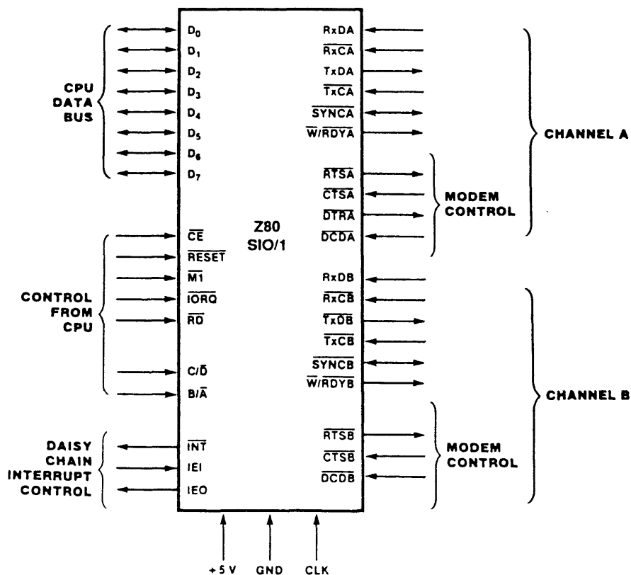
Figure 3. Pin Functions
