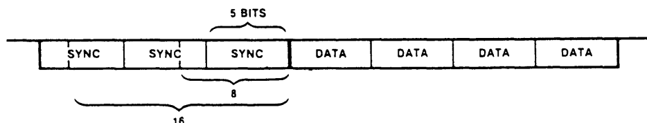
Figure 10. Data Communication
