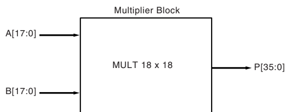
Figure 37: Multiplier Block
