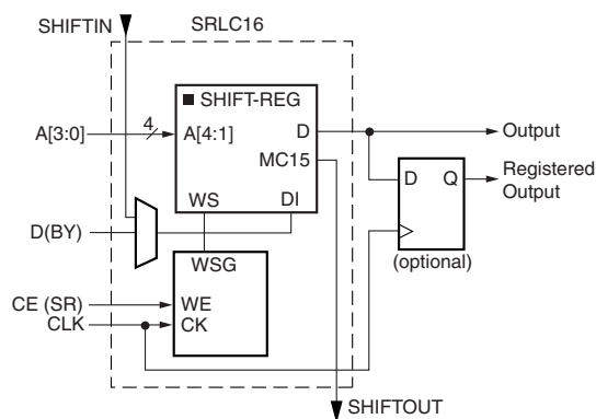
Figure 22: Shift Register Configurations
