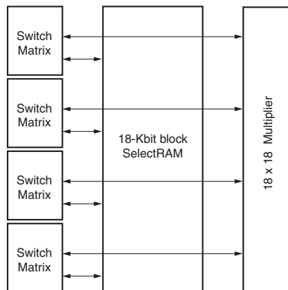
Figure 36: SelectRAM and Multiplier Blocks
