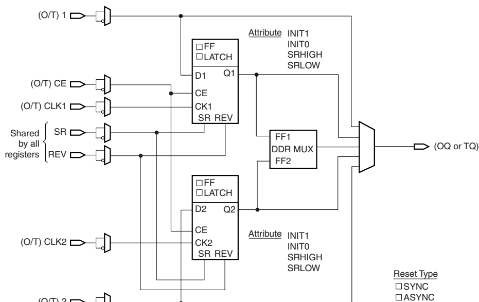
Figure 5: Register/Latch Configuration in an IOB Block
