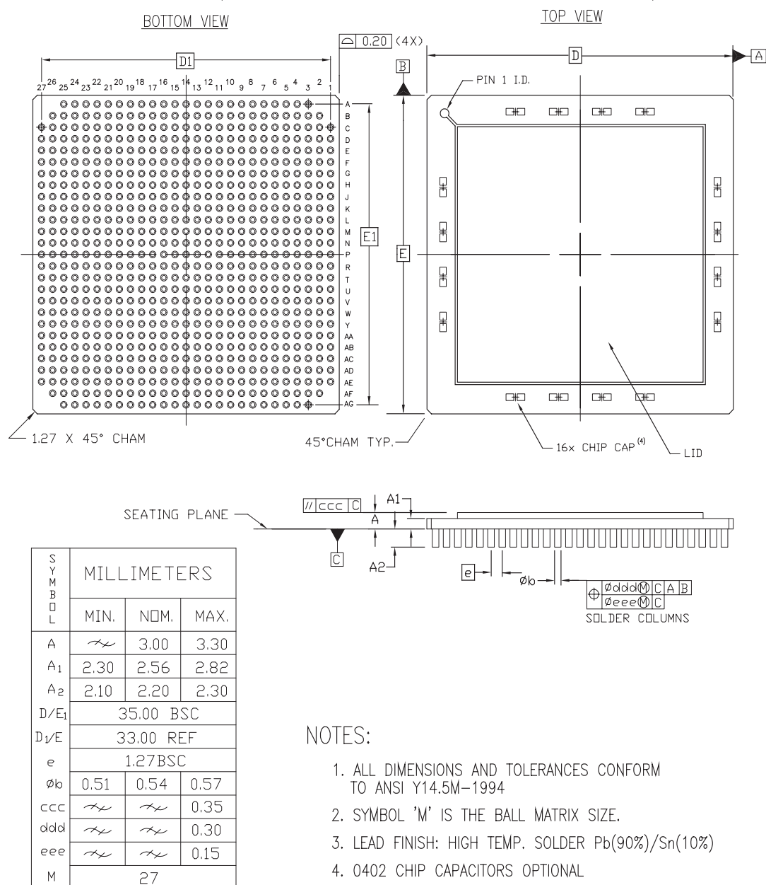
Figure 55: CG717 Ceramic CGA Package Specifications
