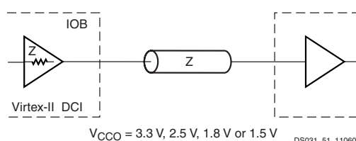
Figure 11: Internal Series Termination
