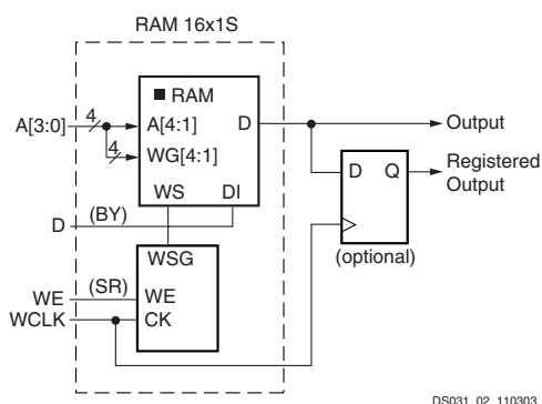
Figure 19: Distributed SelectRAM (RAM16x1S)
