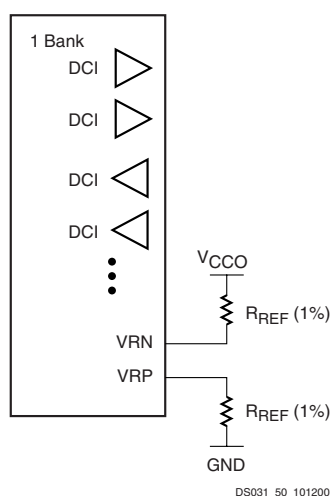
Figure 10: DCI in a Virtex-II Bank
