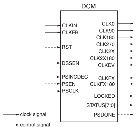
Figure 46: Digital Clock Manager
