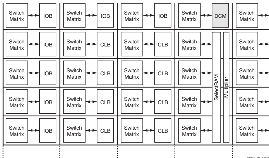
Figure 49: Routing Resources
