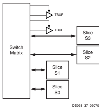
Figure 28: Virtex-II 3-State Buffers
