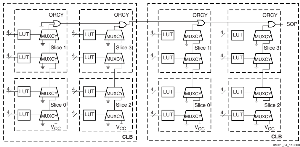
Figure 26: Horizontal Cascade Chain
