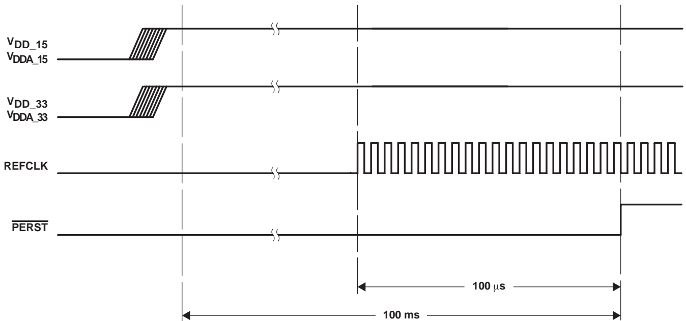
Figure 3–2. Power-Up Sequence
