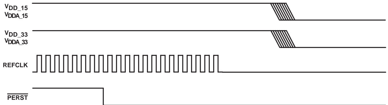
Figure 3–3. Power-Down Sequence
