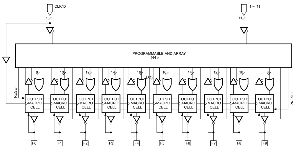
Figure 2: Functional Diagram
