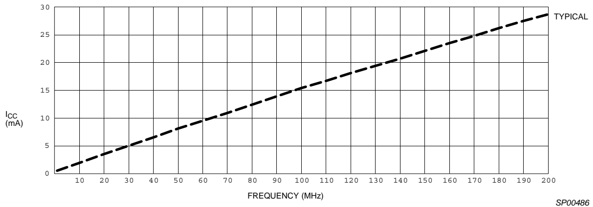
Figure 5: Typical I_{CC} vs. Frequency @ V_{CC} = 5V , 25^{\circ}C (10-bit counter)
