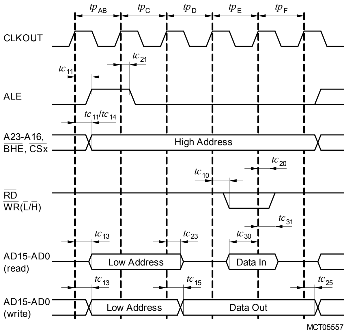
Figure 21 Multiplexed Bus Cycle
