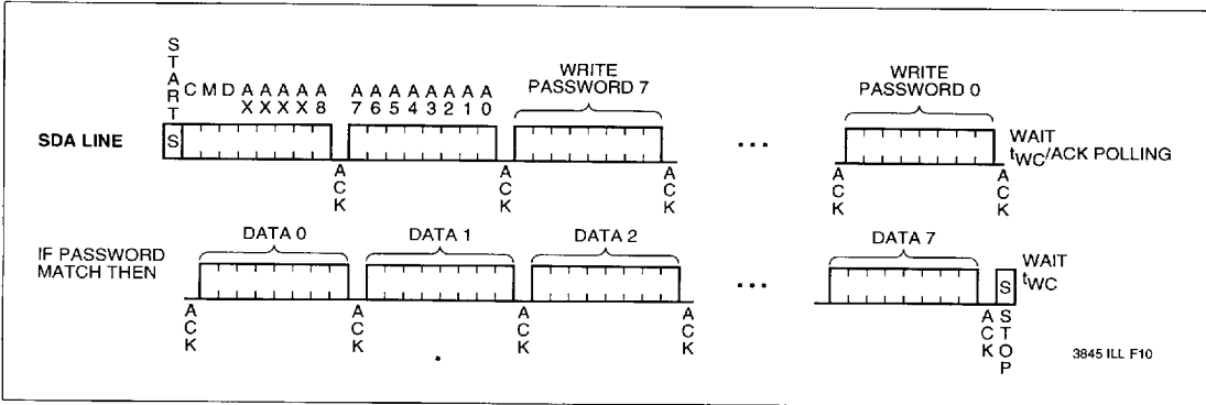
Figure 5. Page Write
