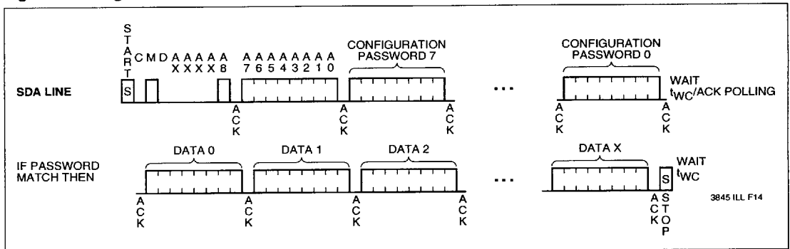
Figure 9. Configuration Write
