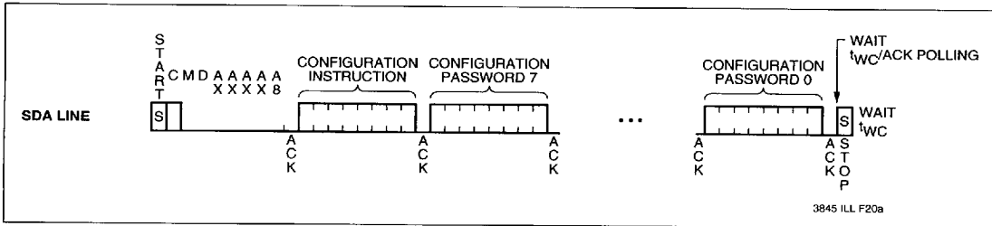
Figure 16. Mass Program/Erase
