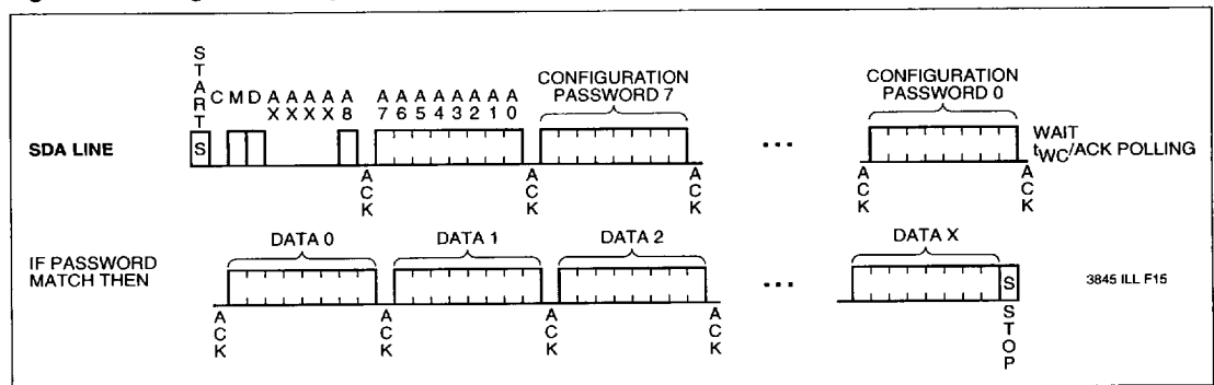
Figure 10. Configuration Sequential Read
