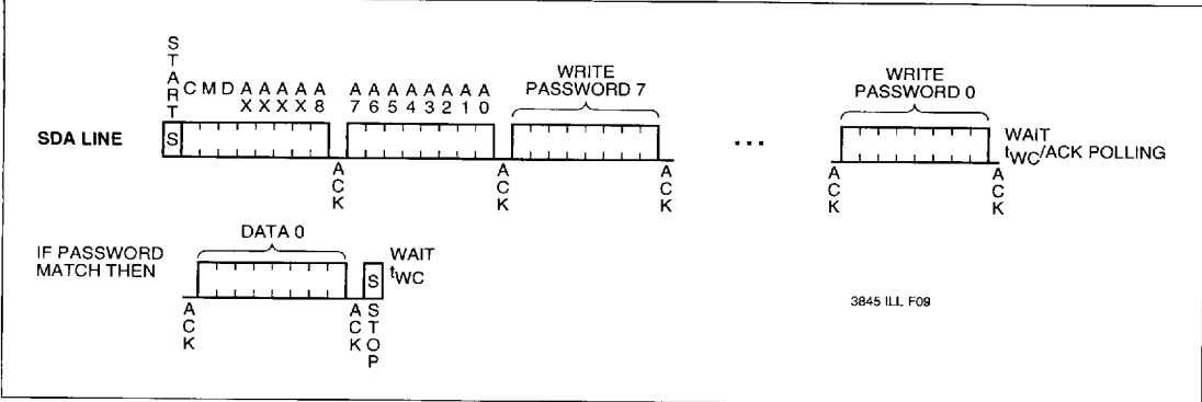
Figure 4. Byte Write
