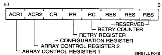
Figure 3. Configuration Registers
