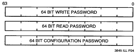
Figure 2. Password Registers
