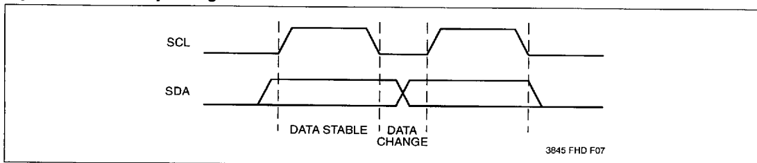
Figure 2. Data Validity During Write
