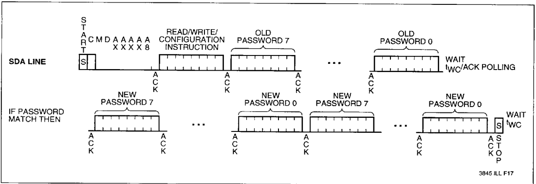
Figure 12. Program Passwords
