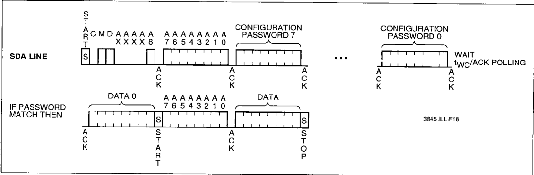
Figure 11. Configuration Random Read
