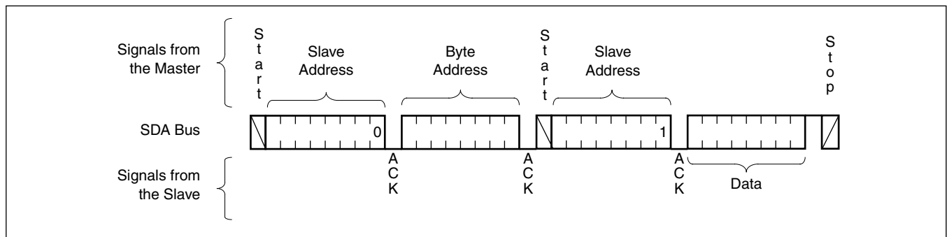
Figure 10. Random Address Read Sequence
