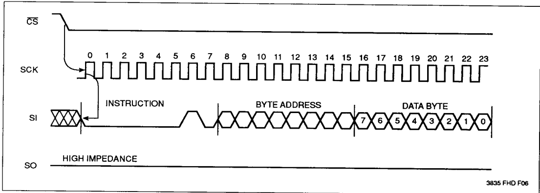
Figure 3. Write Operation Sequence
