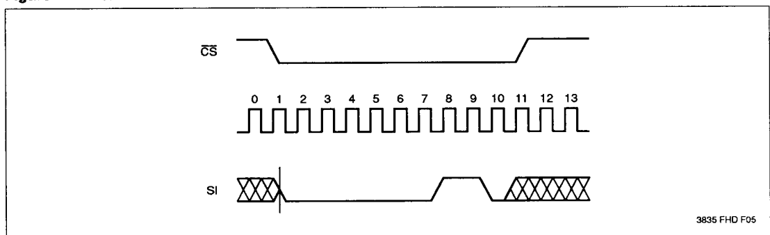
Figure 2. Write Enable Latch
