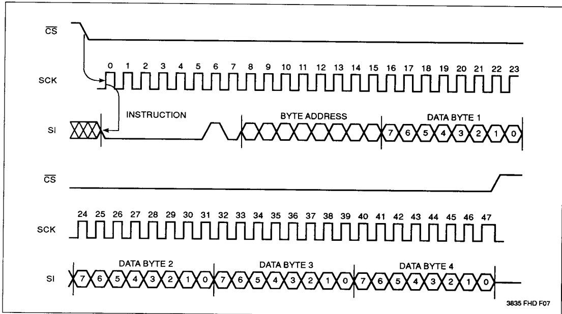
Figure 4. Page Write Operation Sequence
