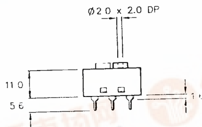
0.8 x 5.0 PCB TERMINALS
