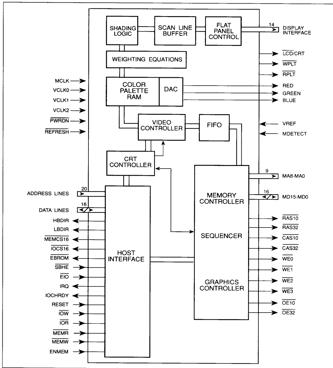
FIGURE 2-1. WD90C22 BLOCK DIAGRAM
