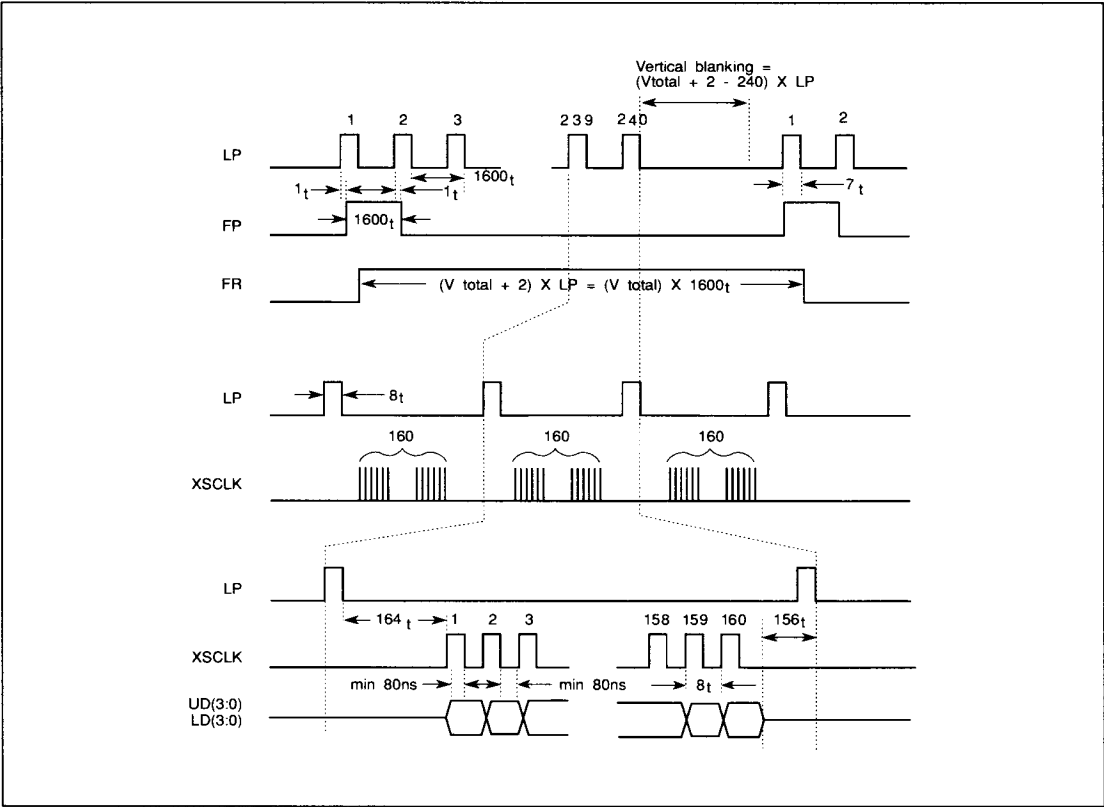
FIGURE C-12. WD90C22 LCD TIMING DIAGRAM ( t=VCLK )
