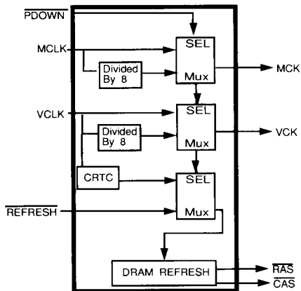
DISPLAY IDLE MODE (SUSPEND/RESUME)
