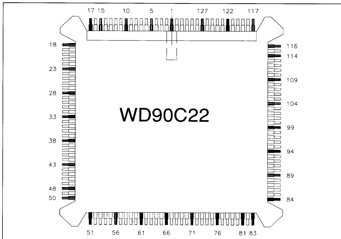
FIGURE 4-1. 132-PIN PQFP PIN ASSIGNMENTS
