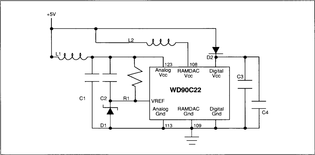
FIGURE 4-2. POWER DISTRIBUTION FOR WD90C22
