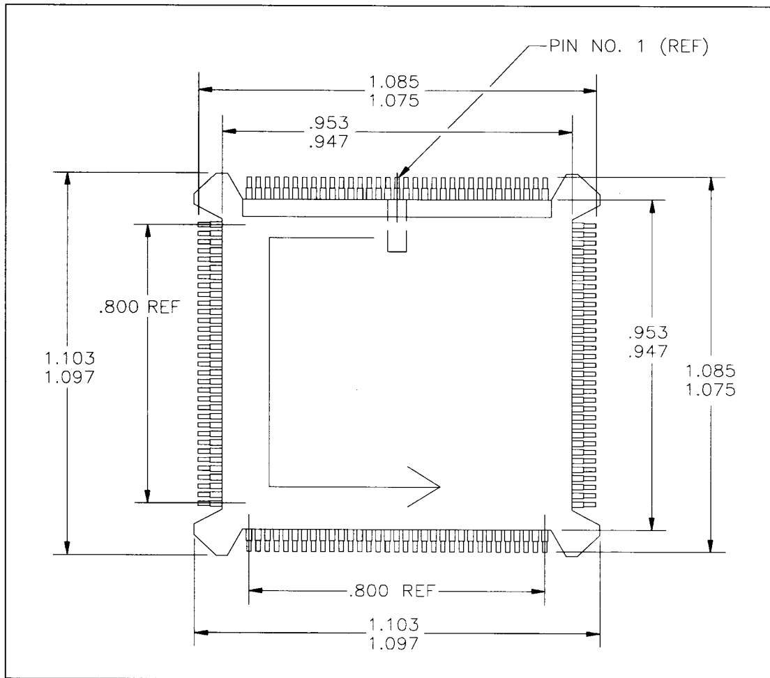
FIGURE D-1. 132-PIN PQFP PACKAGE DIMENSIONS
