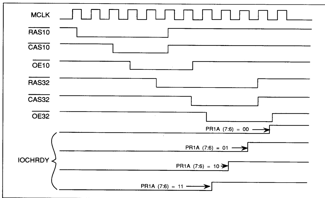
FIGURE C-20. IOCHRDY RELEASE TIMING IN MEMORY READ CYCLE
