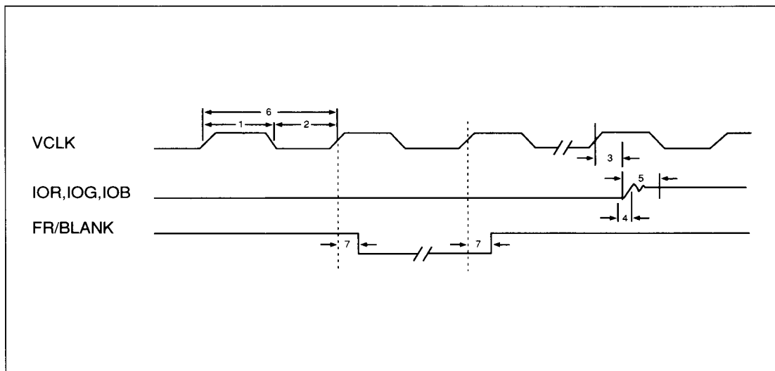
FIGURE C-13. RAMDAC TIMING
