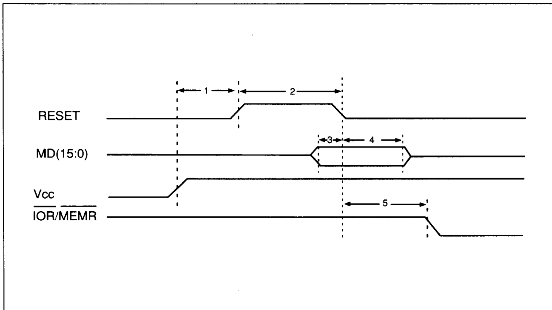
FIGURE C-15. RESET TIMING
