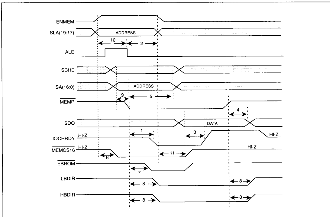
FIGURE C-4. MEMORY READ - AT MODE
