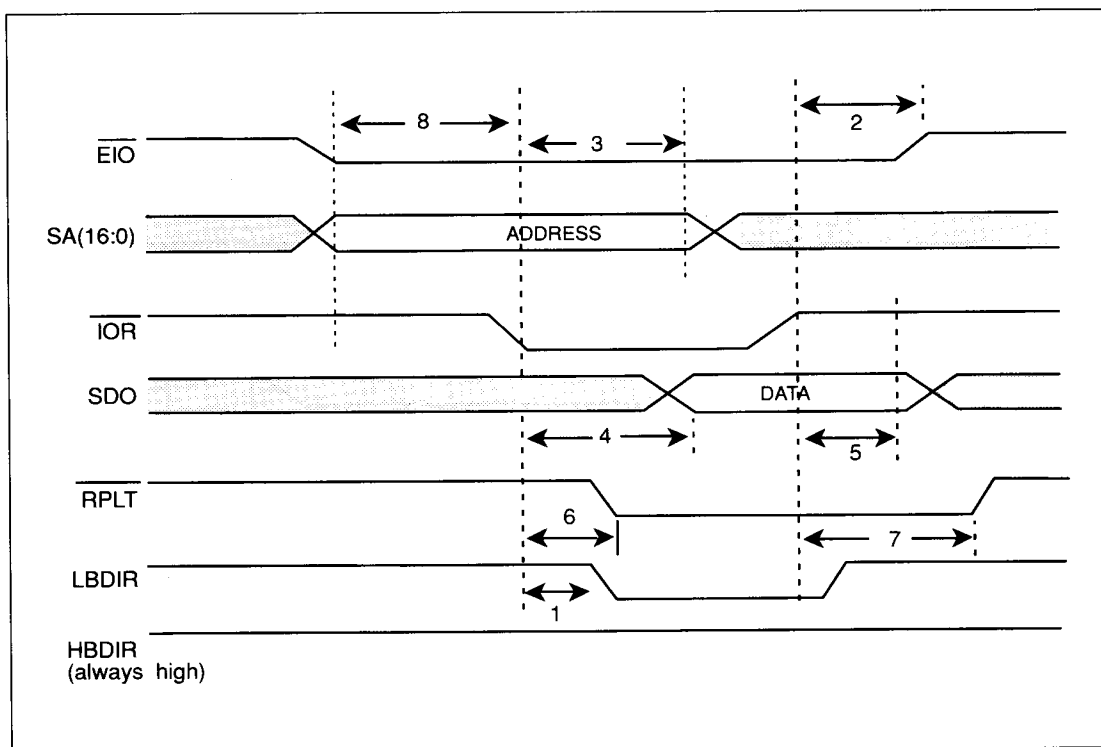
FIGURE C-2. I/O READ-AT MODE
