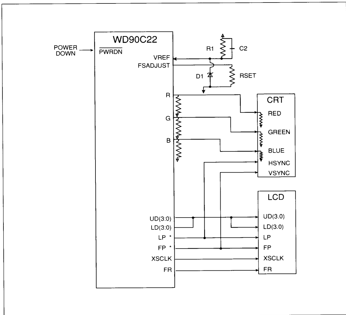
FIGURE A-3. WD90C22 DISPLAY INTERFACE
