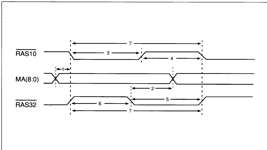
FIGURE C-16. RAS ONLY DRAM REFRESH TIMING
