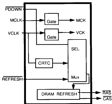
SYSTEM POWER DOWN MODE (SLEEP)
