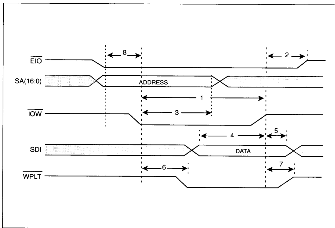
FIGURE C-1. I/O WRITE-AT MODE
