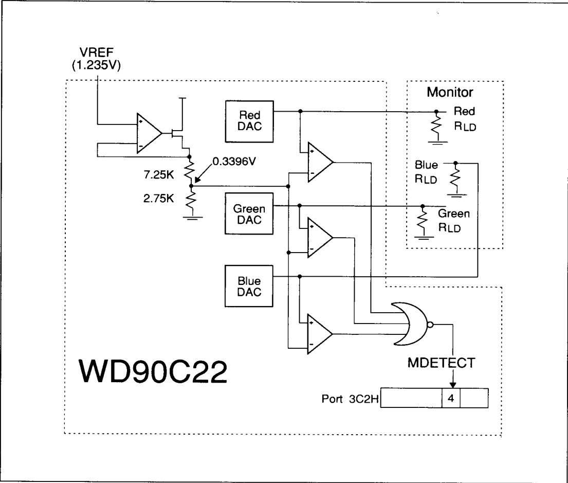
FIGURE B-1. MONITOR DETECTION FOR INTERNAL RAMDAC
