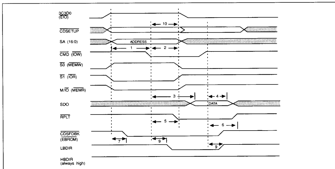
FIGURE C-6. I/O READ - MICRO CHANNEL MODE
