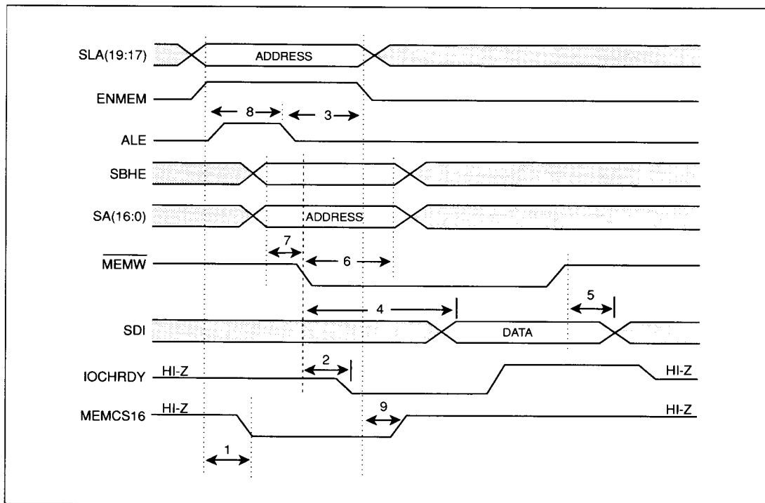
FIGURE C-3. MEMORY WRITE - AT MODE
