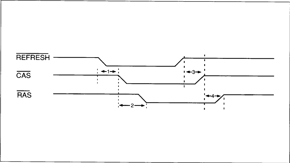
FIGURE C-18. CAS BEFORE RAS REFRESH (Power-Down Mode)
