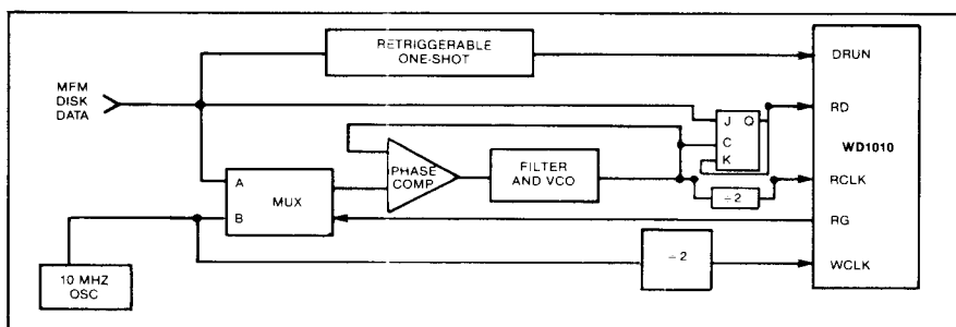
FIGURE 3. DATA RECOVERY CIRCUIT
