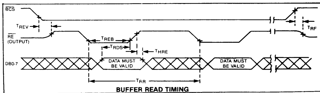
BUFFER READ TIMING
