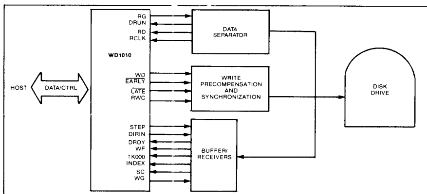
FIGURE 2. DRIVE INTERFACE BLOCK DIAGRAM
