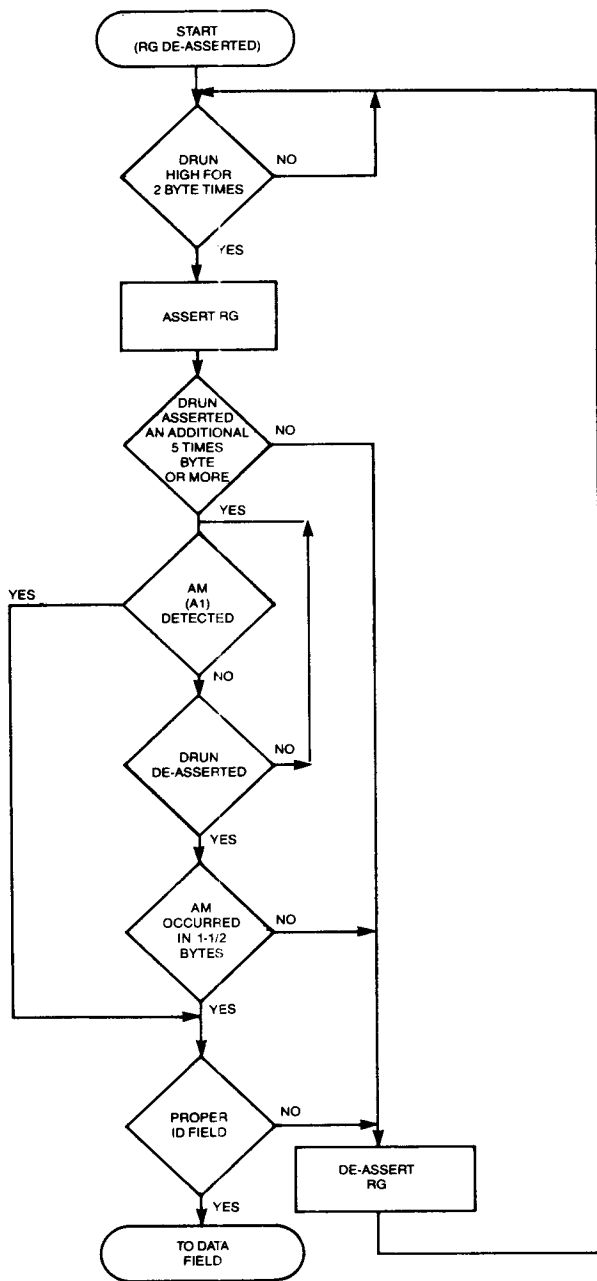
FIGURE 4. PLL CONTROL SEQUENCE FOR ID FIELD
