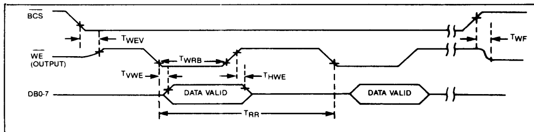
BUFFER WRITE TIMING
