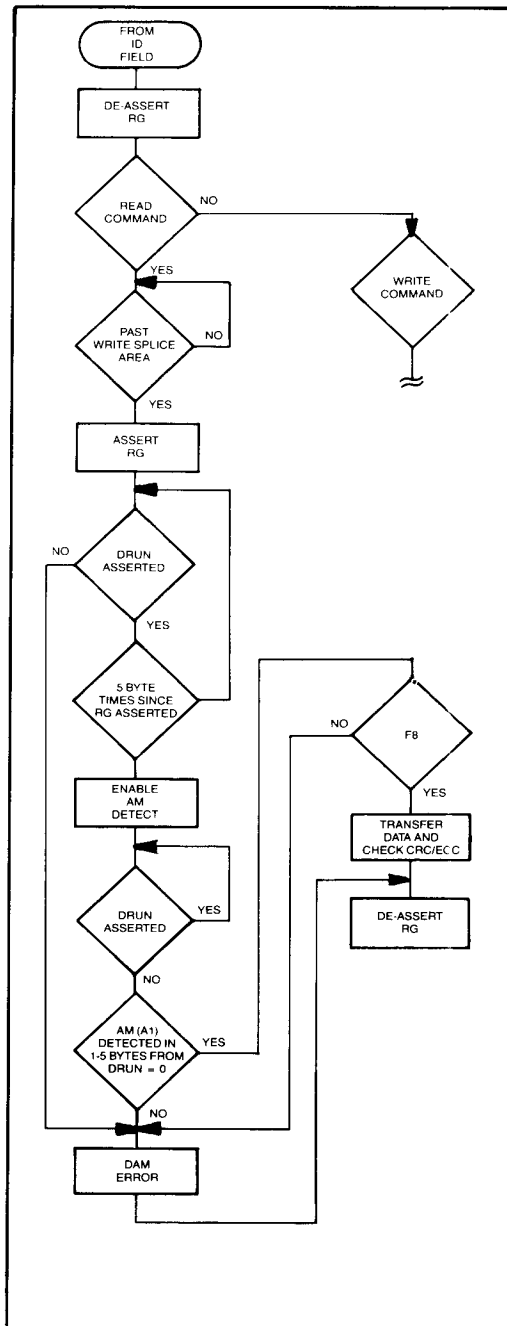
FIGURE 4. (CONT.) PPL CONTROL SEQUENCE FOR DATA FIELD
