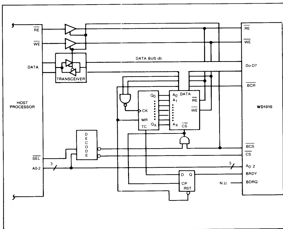
FIGURE 5. HOST INTERFACE
