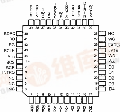
QUAD PIN DESIGNATION
