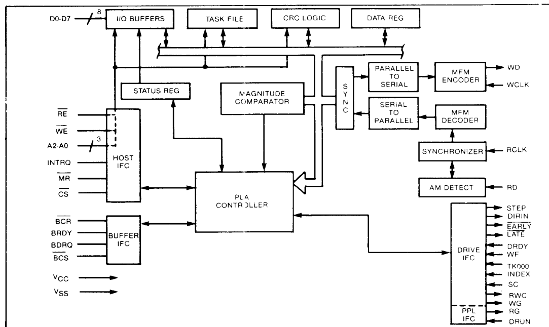
FIGURE 1. WD1010 BLOCK DIAGRAM
