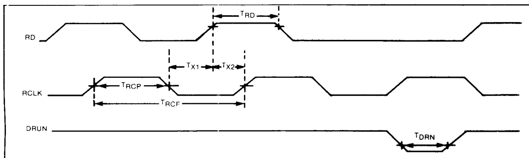
READ DATA TIMING
