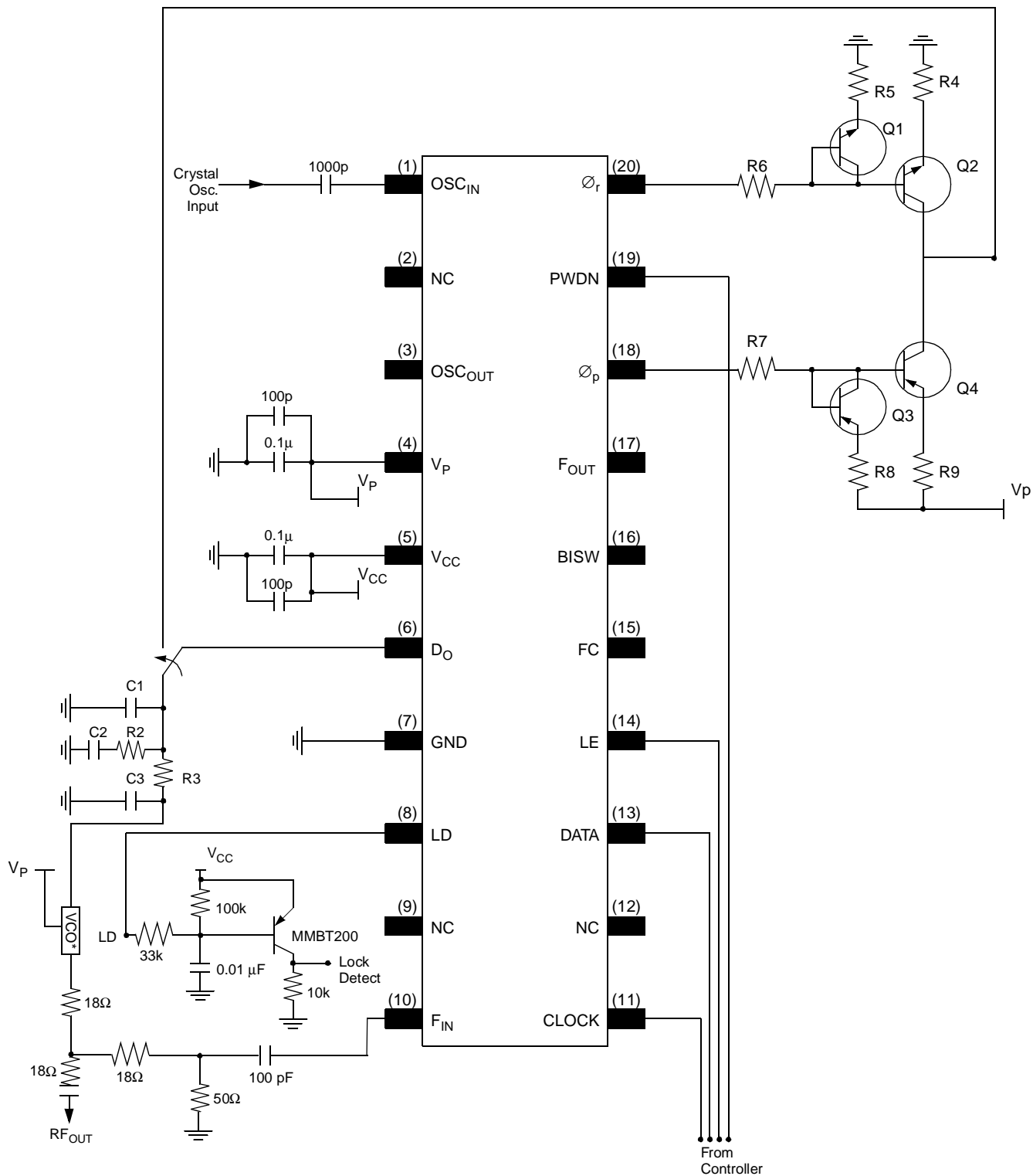
Figure 1. Application Diagram Example - WB1220 2.0-GHz PLL
