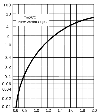
FIG.4-TYPICAL FORWARD CHARACTERISTIC
