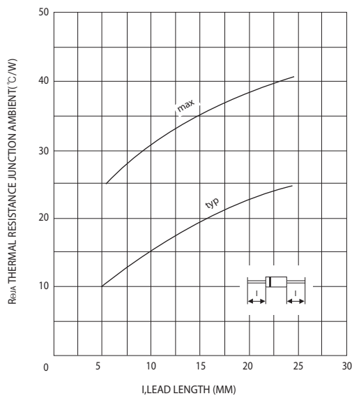
FIG.3-TYPICAL THERMAL IMPEDANCE
