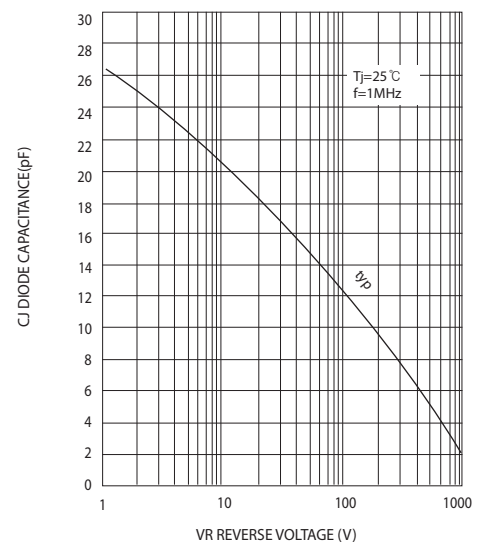
FIG.4-TYPICAL JUNCTION CAPACITANCE
