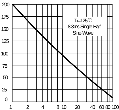
FIG.3 –PEAK FORWARD SURGE CURRENT
