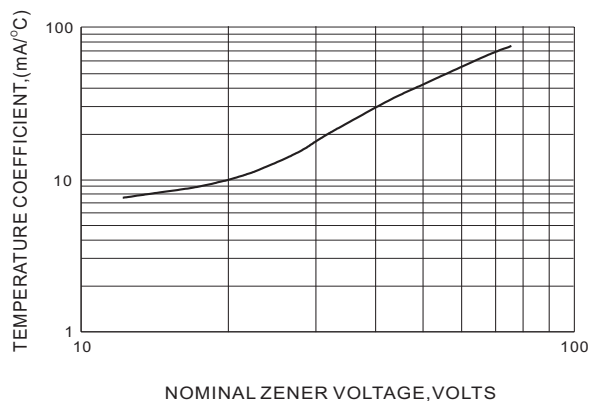
Fig.2 TEMPERATURE COEFFICIENTS
