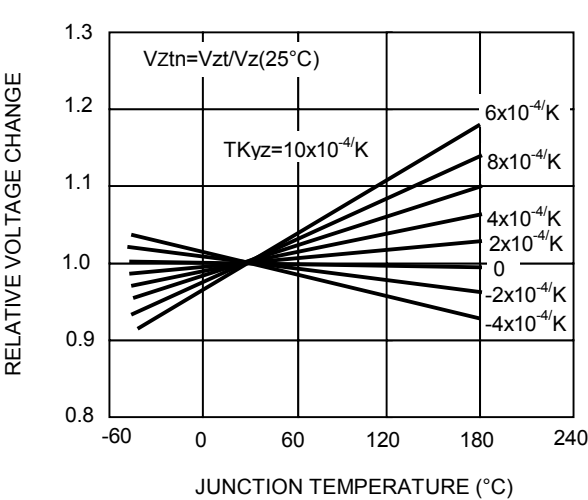
FIG. 4 - TYPICAL CHANGE OF WORKING VOLTAGE VS. JUNCTION TEMPERATURE
