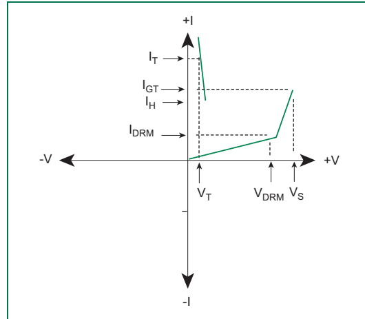
V-I Characteristics for Positive Batrax
