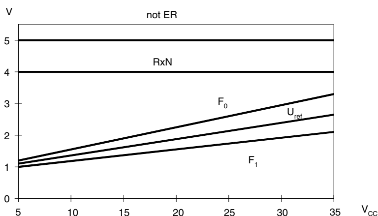
Figure 7-1. Comparator Thresholds
