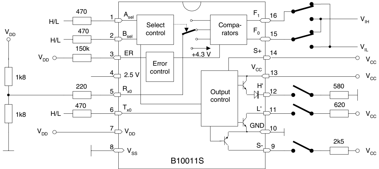
Figure 6-2. Application Circuit
