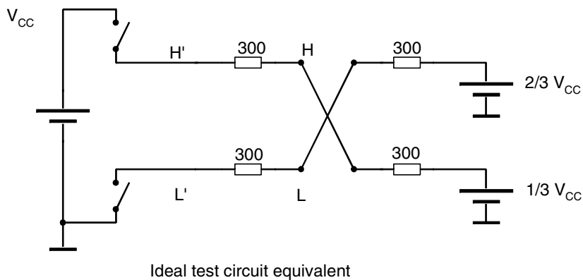
Figure 7-2. Test Circuit Equivalent
