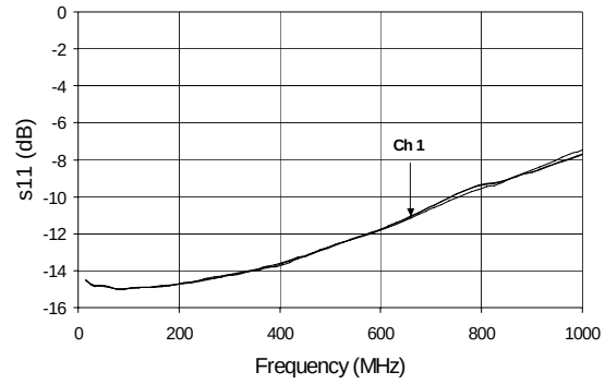
Input Return Loss Vs. Freq
