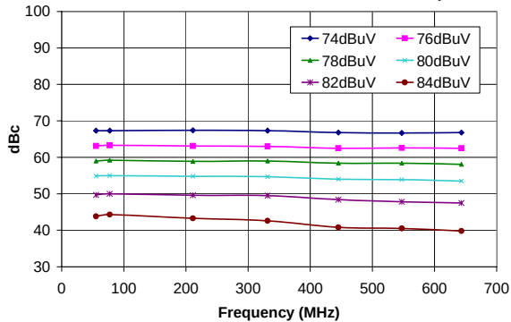
CGA-0116 Ch. 1 & 2: XMOD vs. Pin and Freq.
