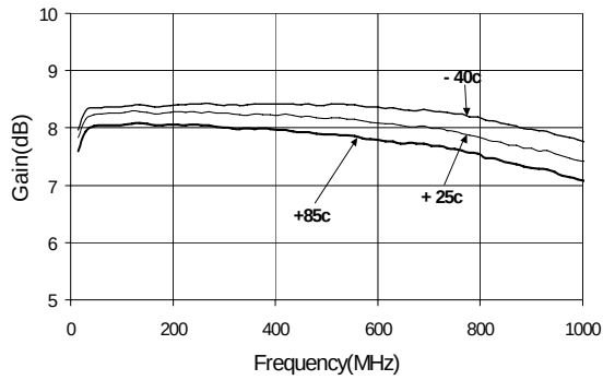
Ch 3 Gain vs Temperature
