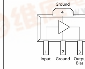
Functional Block Diagram (SOT-89)
