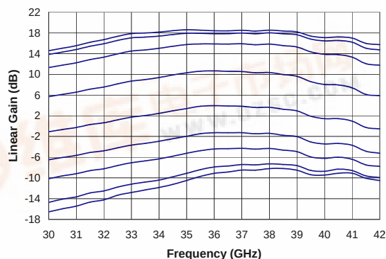
On-Wafer Measurements
