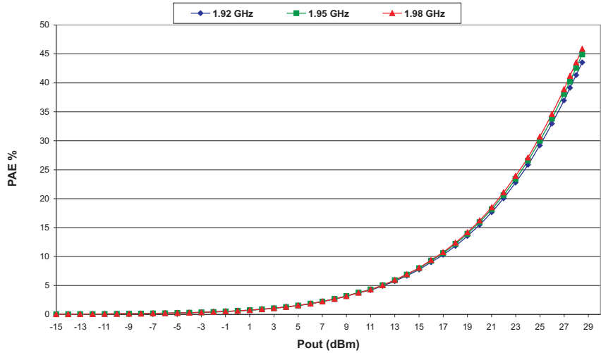
Figure 20: PAE vs P_{OUT} ( T = +25\text{ }^{\circ}\text{C} , V_{CC} = 3.4\text{ V} , V_{REF} = 2.85\text{ V} , V_{MODE} = 1.5 + 0.025 \cdot P_{OUT} )
