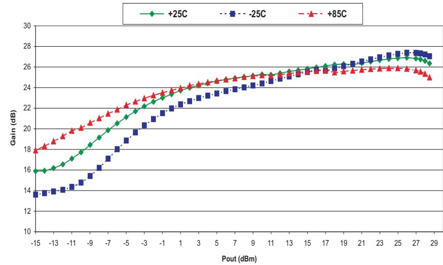
Figure 25: Gain vs P_{OUT} ( V_{CC} = 3.4\text{ V} , V_{REF} = 2.85\text{ V} , V_{MODE} = 1.5 + 0.025 \cdot P_{OUT} , F = 1.95\text{ GHz} )
