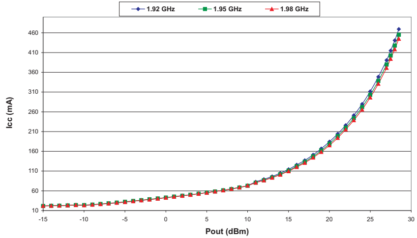
Figure 19: I_{CC} vs P_{OUT} ( T = +25\text{ }^{\circ}\text{C} , V_{CC} = 3.4\text{ V} , V_{REF} = 2.85\text{ V} , V_{MODE} = 1.5 + 0.025 \cdot P_{OUT} )
