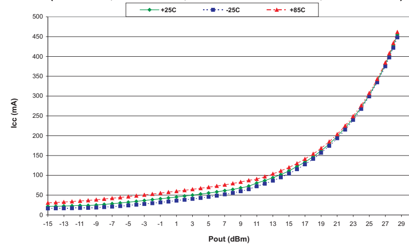
Figure 24: I_{CC} vs P_{OUT} ( V_{CC} = 3.4\text{ V} , V_{REF} = 2.85\text{ V} , V_{MODE} = 1.5 + 0.025 \cdot P_{OUT} , F = 1.95\text{ GHz} )
