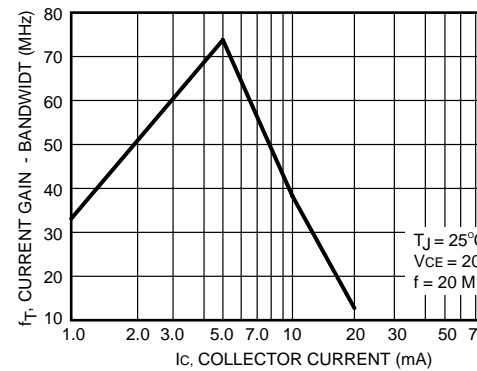
Figure 3. Current-Gain - Bandwidth
