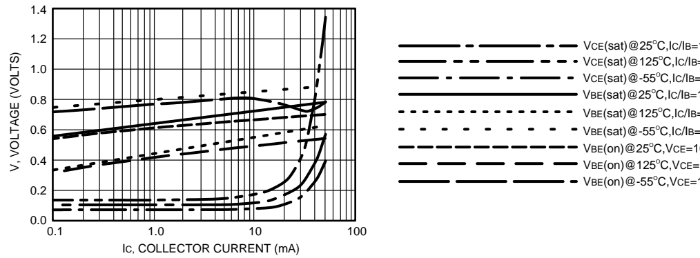
Figure 4. "ON" Voltages
