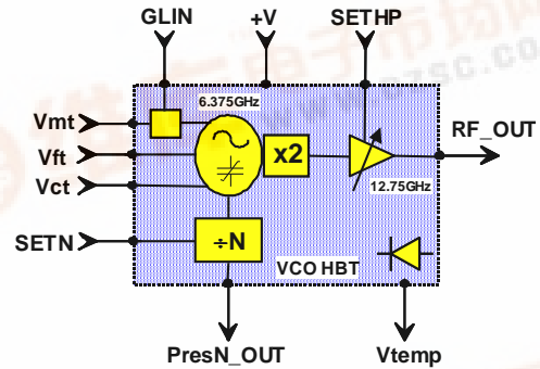
VCO multifunction block diagram
