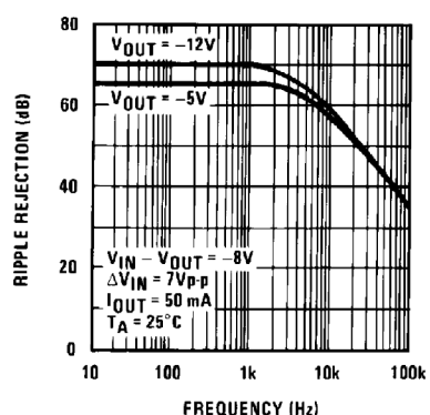
Ripple Rejection
