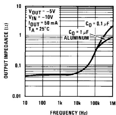
Output Impedance
