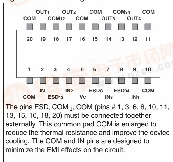
Figure 1. Pin configuration
