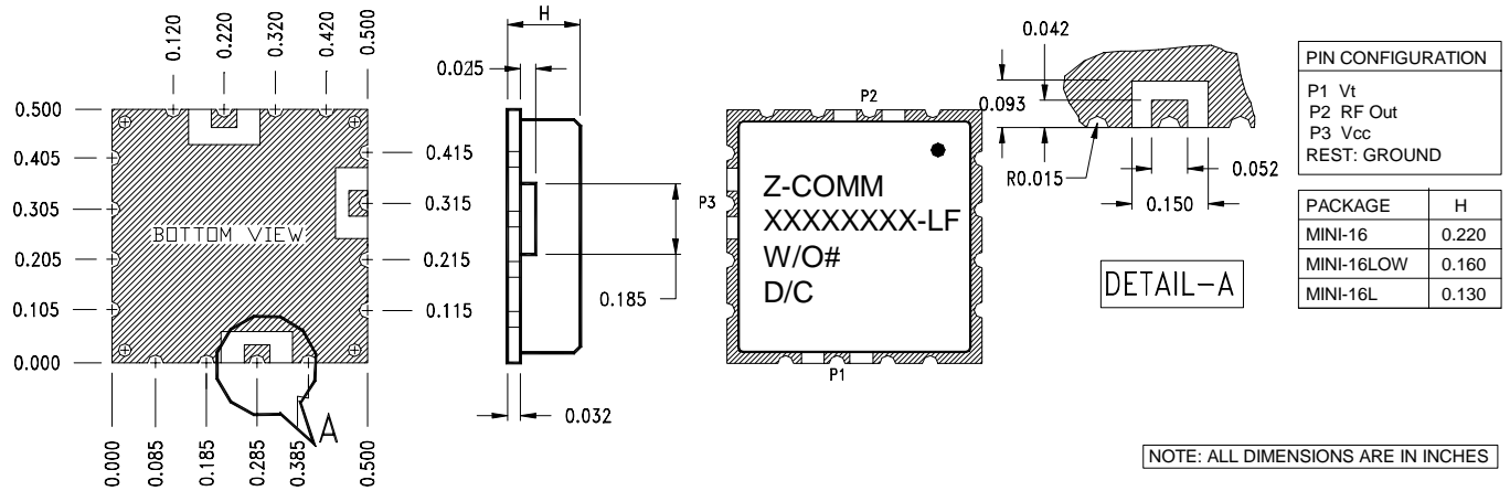
PHYSICAL DIMENSIONS
