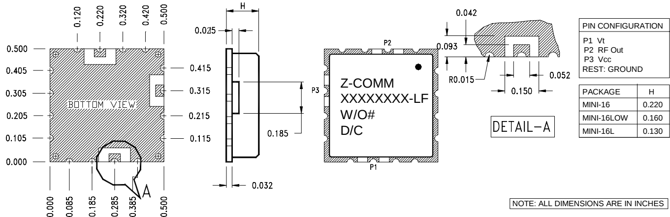
PHYSICAL DIMENSIONS
