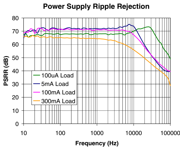
Figure 26. Power Supply Ripple Rejection ( C_{OUT}=2.2\mu F , C_{BYF}=100nF )
