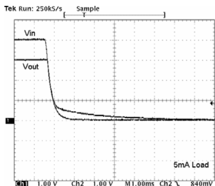
Figure 24. Power-Down ( I_{LOAD} = 5mA )
