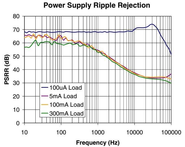
Figure 27. Power Supply Ripple Rejection (No C_{OUT} , C_{BYF}=100nF )
