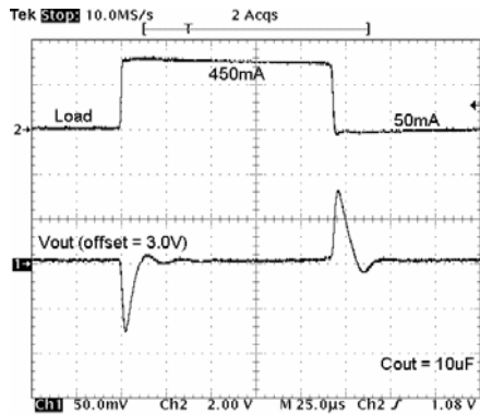
Figure 13. 10% to 90% Load Step ( t_r=1\mu s , C_{OUT}=10\mu F )
