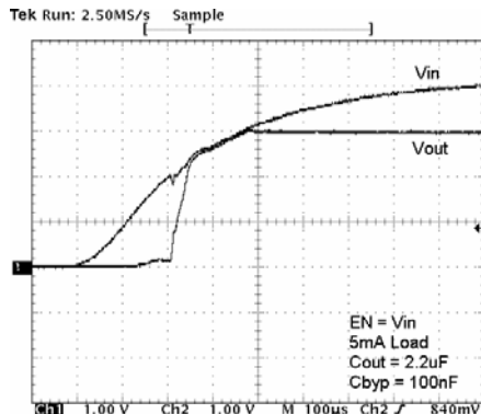
Figure 23. Power-Up ( EN = V_{IN} , I_{LOAD} = 5mA , C_{OUT} = 2.2\mu F , C_{BYP} = 100nF )
