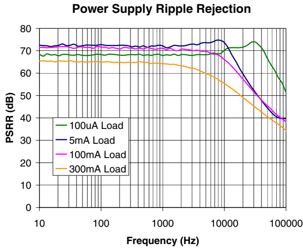
Figure 25. Power Supply Ripple Rejection ( C_{OUT}=10\mu F , C_{BYF}=100nF )
