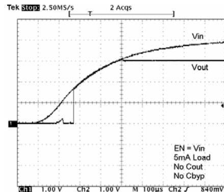
Figure 22. Power-Up ( EN = V_{IN} , I_{LOAD} = 5mA , No C_{OUT} , No C_{BYP} )
