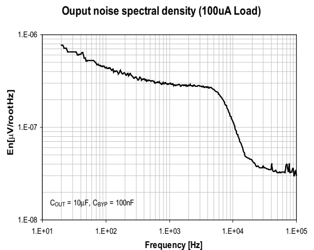
Figure 28. Output Noise Spectral Density ( I_{LOAD}=100\mu A , C_{OUT}=10\mu F , C_{BYF}=100nF )
