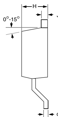
Package Dimensions for TO252-5
