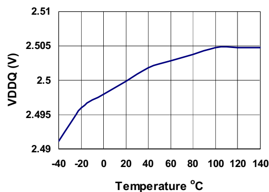
VDDQ vs. Temperature
