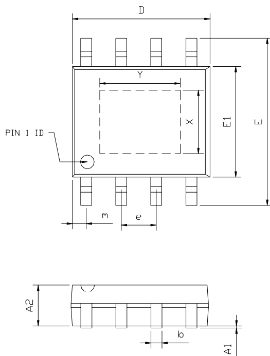
8-Pin SOP w/ Power Pad (PS08)
