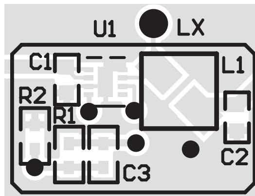
Figure 3: Exploded View of AAT1120 Evaluation Board Top Side Layout.
