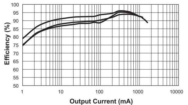
AAT1151 Efficiency (V OUT = 2.5V; L = 4.2µH)
