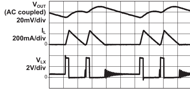
Light Load Switching Waveform (LL Mode; V_{IN} = 4.2V ; V_{OUT} = 0.6V ; R_L = 10\Omega ; C_{OUT} = 4.7\mu F ; L = 2.2\mu H )
