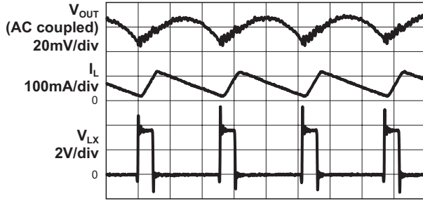
Light Load Switching Waveform (PWM Mode; V_{IN} = 4.2V ; V_{OUT} = 0.6V ; R_L = 10\Omega ; C_{OUT} = 4.7\mu F ; L = 2.2\mu H )
