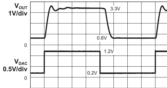
DAC Transient Response in PWM Mode ( V_{IN} = 3.6V ; R_L = 10\Omega ; C_{OUT} = 4.7\mu F ; L = 2.2\mu H )
