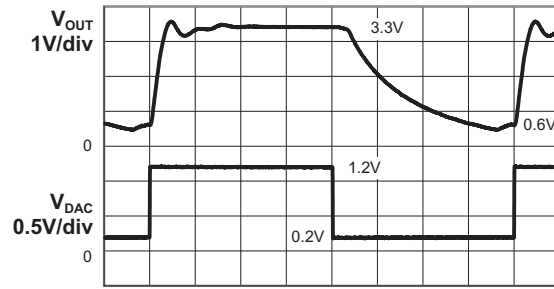
DAC Transient Response in LL Mode ( V_{IN} = 3.6V ; R_L = 10\Omega ; C_{OUT} = 4.7\mu F ; L = 2.2\mu H )
