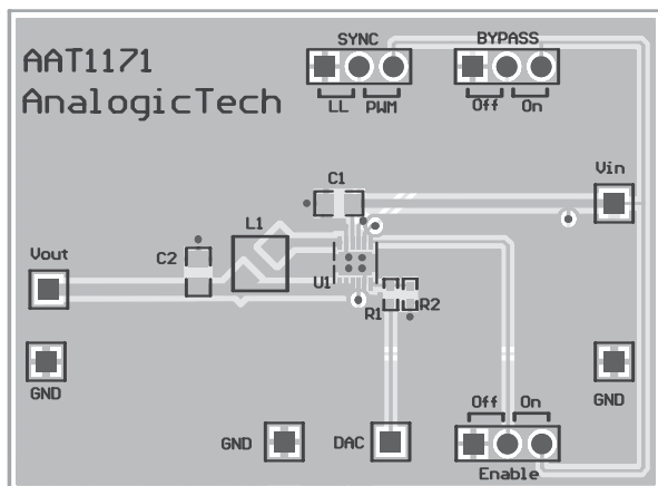
Figure 3: AAT1171 Evaluation Board Top Side Layout.
