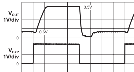
Bypass Transient Response (LL Mode; V_{IN} = 3.6V ; R_L = 10\Omega ; C_{OUT} = 4.7\mu F ; L = 2.2\mu H )
