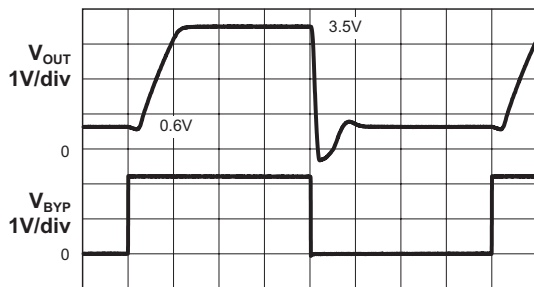
Bypass Transient Response (PWM Mode; V_{IN} = 3.6V ; R_L = 10\Omega ; C_{OUT} = 4.7\mu F ; L = 2.2\mu H )
