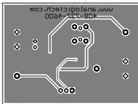
Figure 6: AAT1184ITP Evaluation Board Bottom Layer.
