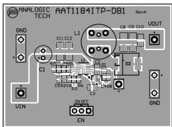
Figure 5: AAT1184ITP Evaluation Board Top Layer.
