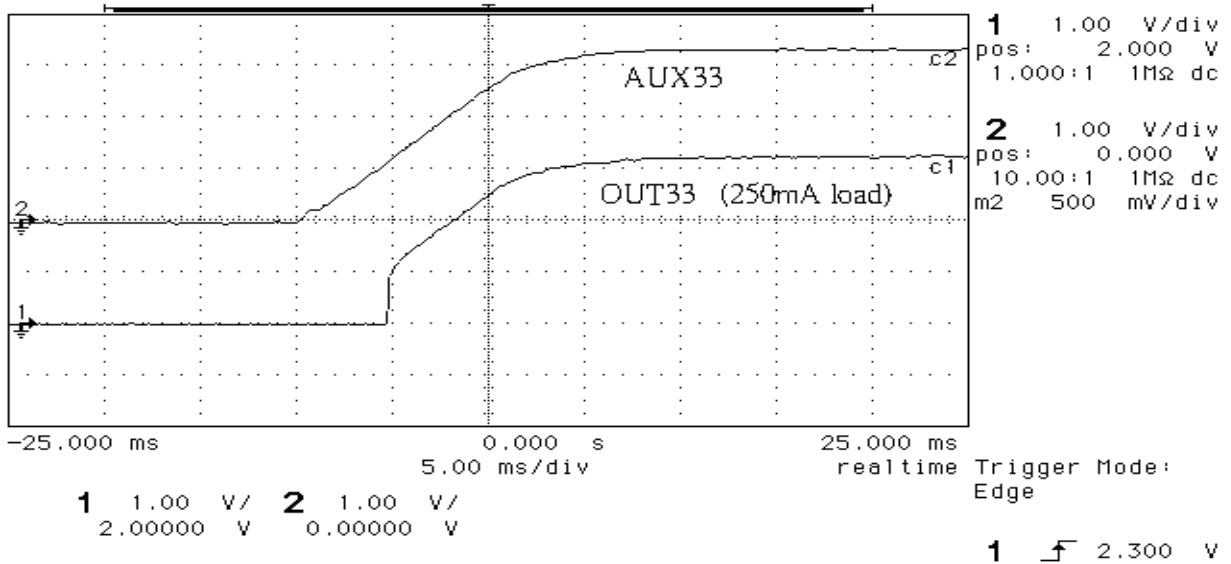
Fig. 3. 3.3V AUX33 Cold Start
