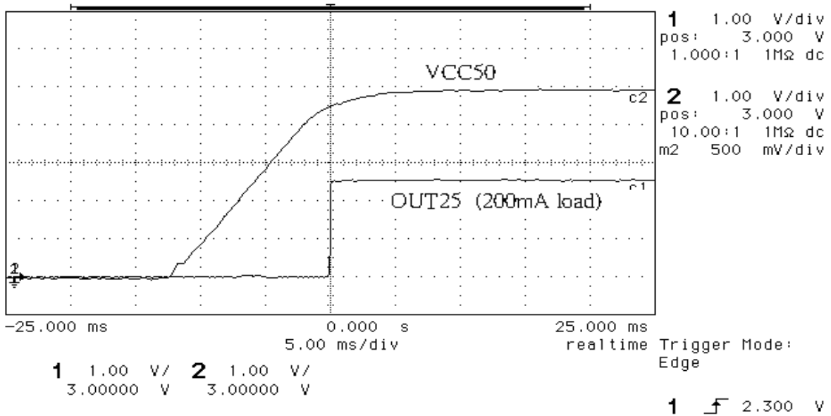
Fig. 2. 2.5V VCC50 Cold Start
