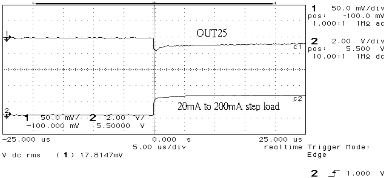
Fig. 18. 2.5V Load Transient Response Rising
