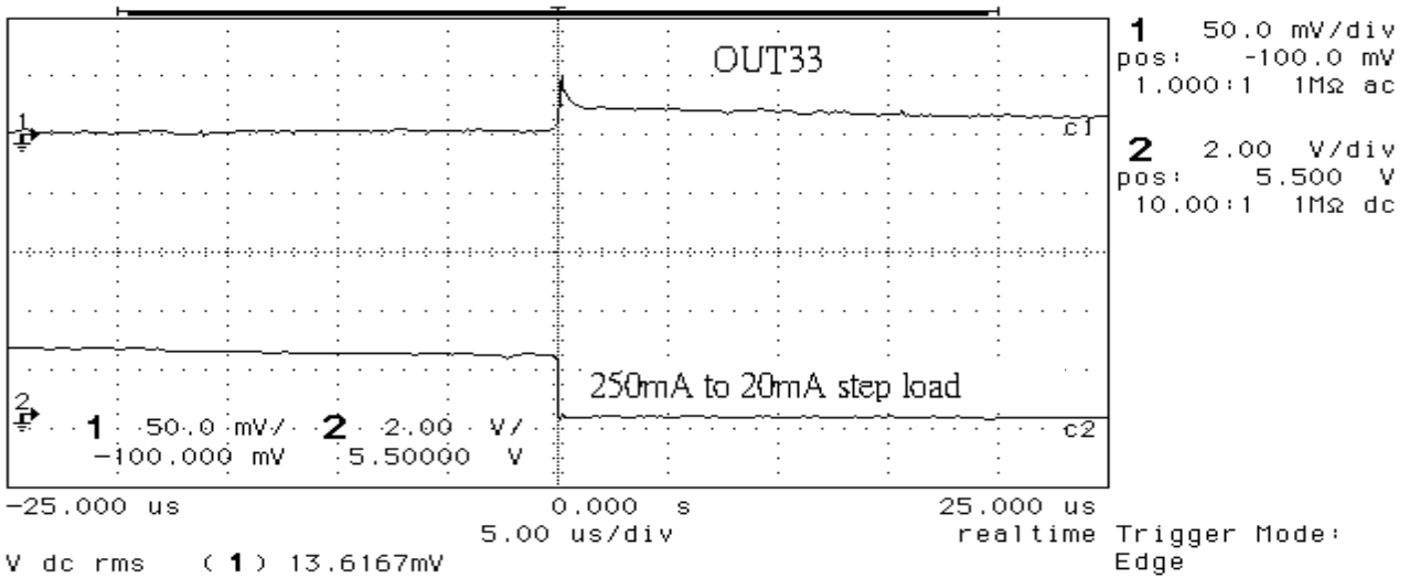
Fig. 15. 3.3V Load Transient Response Falling.
