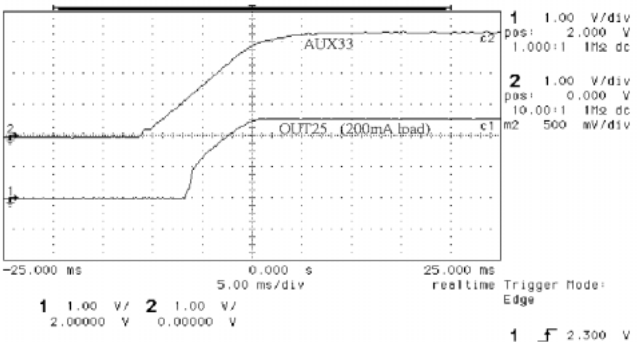
Fig. 4. 2.5V AUX33 Cold Start
