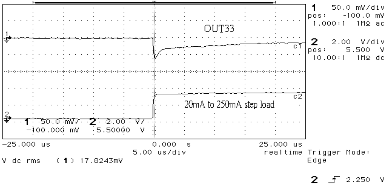
Fig. 17. 3.3V Load Transient Response Rising
