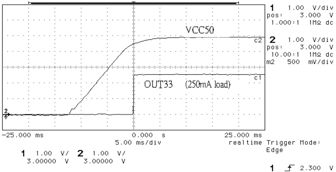
Fig. 1. 3.3V VCC50 Cold Start
