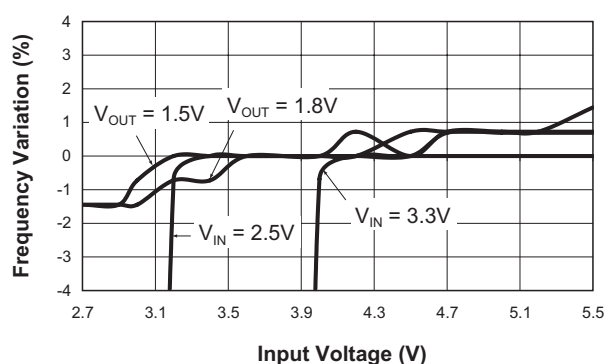
Switching Frequency vs. Input Voltage ( I_{OUT} = 600mA ; 25°C)
