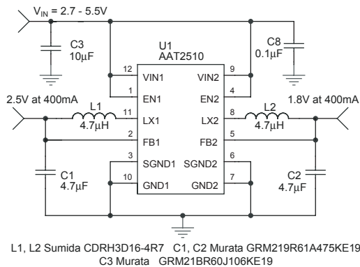
Figure 1: AAT2510 Fixed Output.
