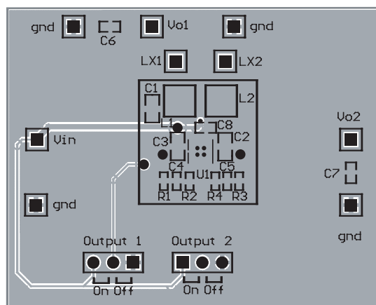
Figure 5: AAT2510 Evaluation Board Bottom Side.
