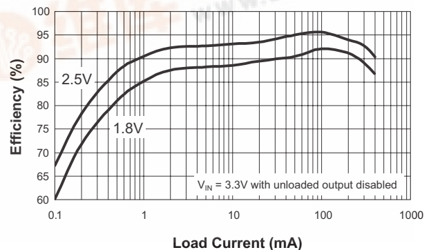
AAT2510 Efficiency
