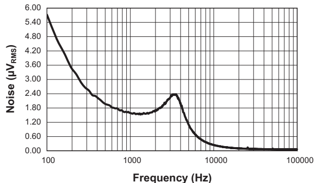
LDO Output Voltage Noise (\text{No Load; Power BW: } 100\sim 100\text{KHz})
