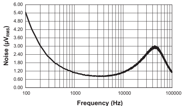
LDO Output Voltage Noise (I_{OUT3} = 10\text{mA, Power BW} = 100\sim 100\text{KHz})
