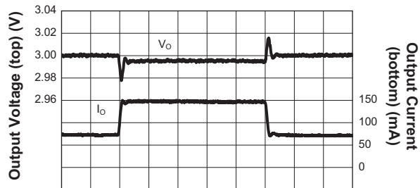
Load Transient Response LDO4 ( I_{OUT4} = 75mA to 150mA ; V_{BAT} = 3.6V ; V_{OUT4} = 3V ; C_{OUT} = 4.7µF )
