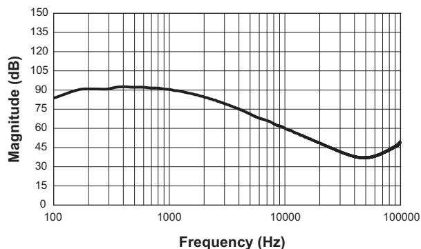
LDO Power Supply Rejection Ratio, PSRR (I_{OUT3} = 10\text{mA, BW} = 100\sim 100\text{KHz})
