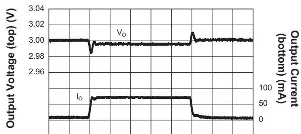
Load Transient Response LDO4 ( I_{OUT4} = 10mA to 75mA ; V_{BAT} = 3.6V ; V_{OUT4} = 3V ; C_{OUT} = 4.7µF )
