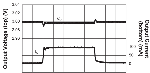
Load Transient Response LDO1 ( I_{OUT1} = 10mA to 100mA ; V_{BAT} = 3.6V ; V_{OUT1} = 3V )
