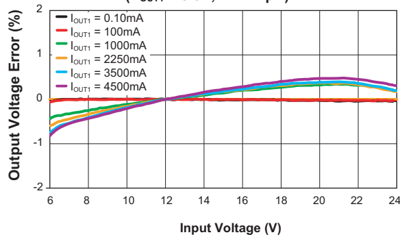
Step-Down Converter Output Voltage Error vs. Input Voltage ( V_{OUT1} = 3.3V ; L = 4.7\mu H )
