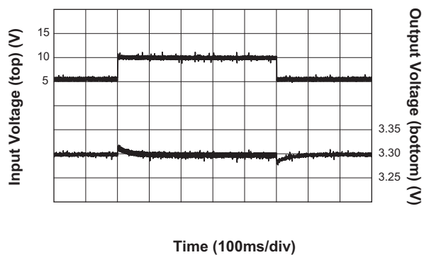
Step-Down Converter Line Transient Response ( V_{IN1} = 6V to 10V ; V_{OUT1} = 3.3V ; I_{OUT1} = 4.5A )
