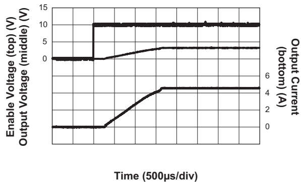
Step-Down Converter Soft Start ( V_{IN1} = 12V ; V_{OUT1} = 3.3V ; I_{OUT1} = 4.5A )
